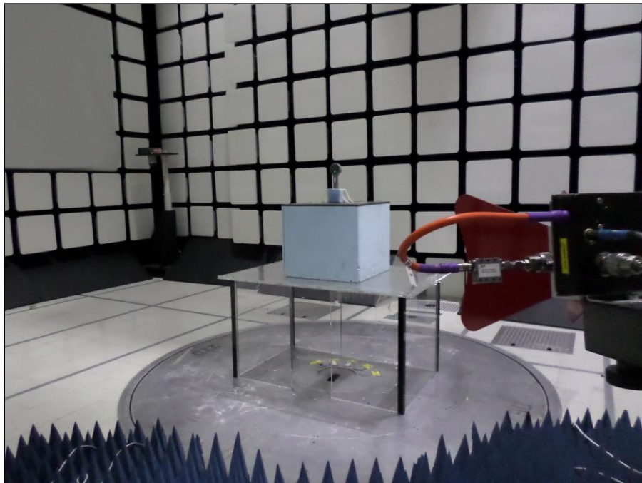
Photograph 3. Radiated Spurious Emissions, 1 – 18 GHz
