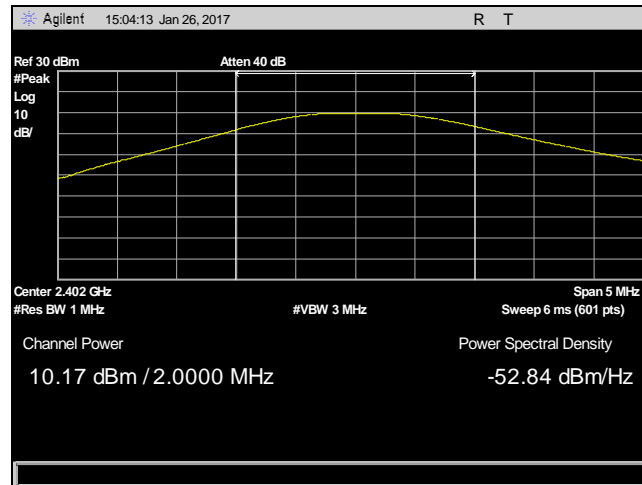
Plot 12. Peak Power Output, Channel Power, BT, 2402 MHz
