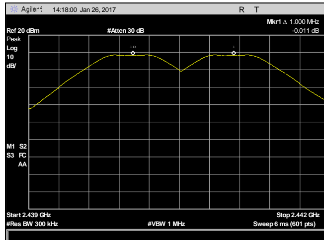
Plot 10. Channel Separation, Mid Channel
