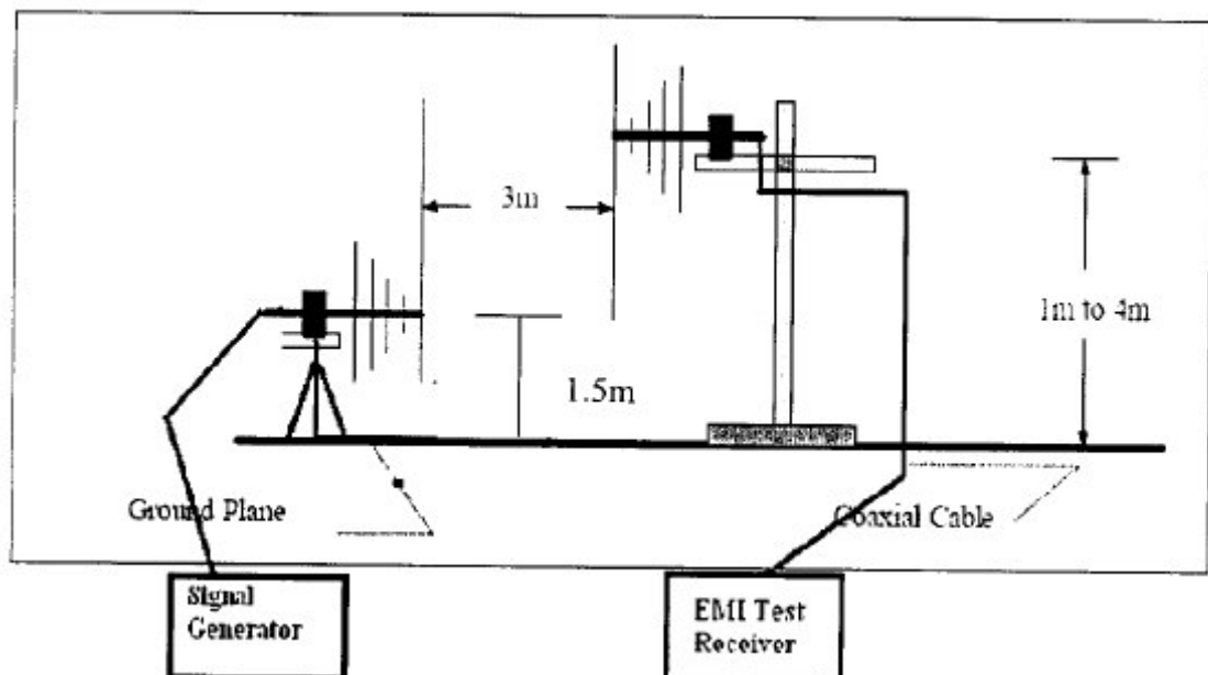
Substitution Method test setup
