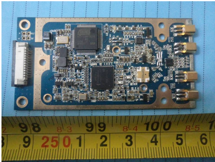
EUT – RF Module Board Top View
