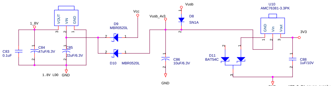
USB 3.3V power supply
