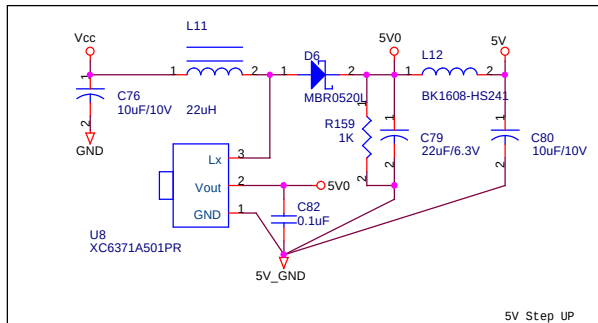
5V Step UP
