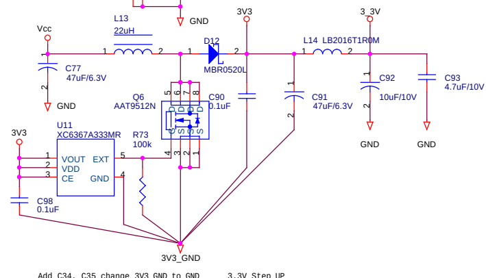
3.3V Step UP
