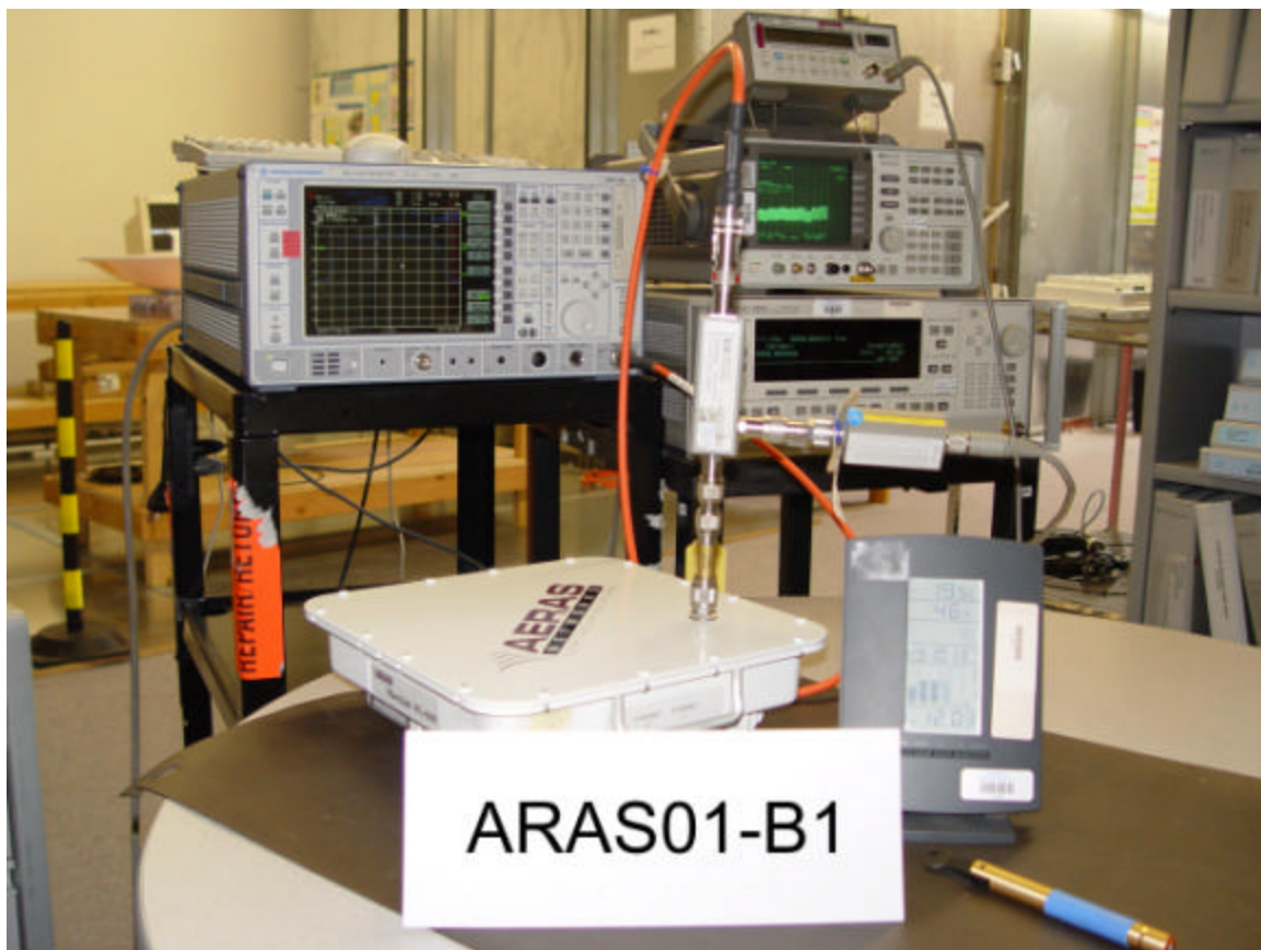
TEST SET UP Conducted Tests
