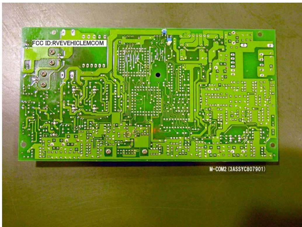
Module (Back side of MCOM-2)
