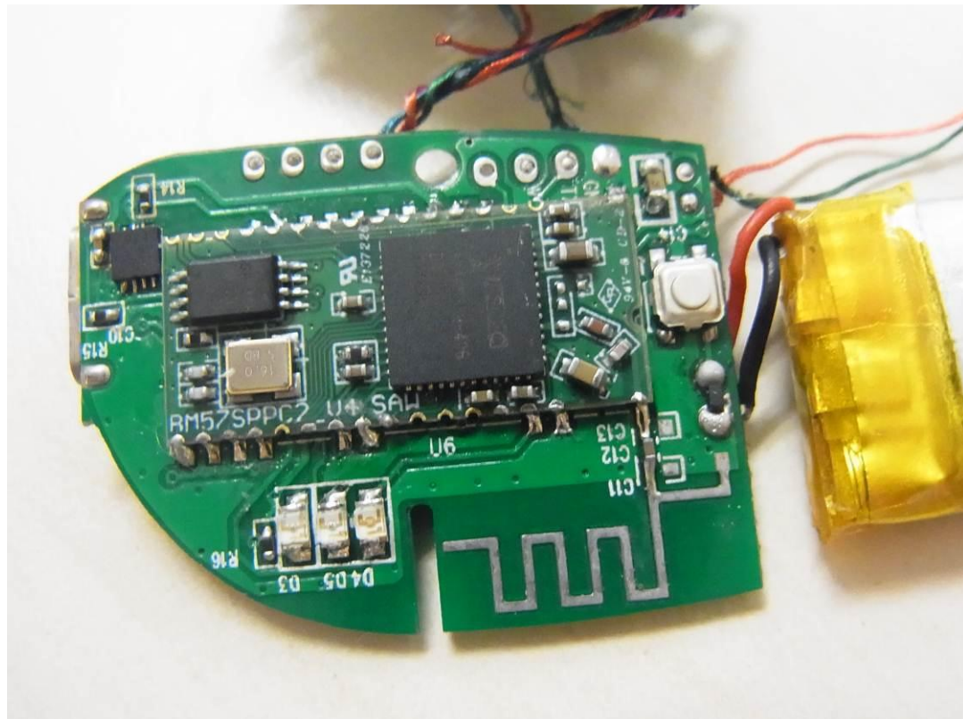
Fig. 6: Internal view
