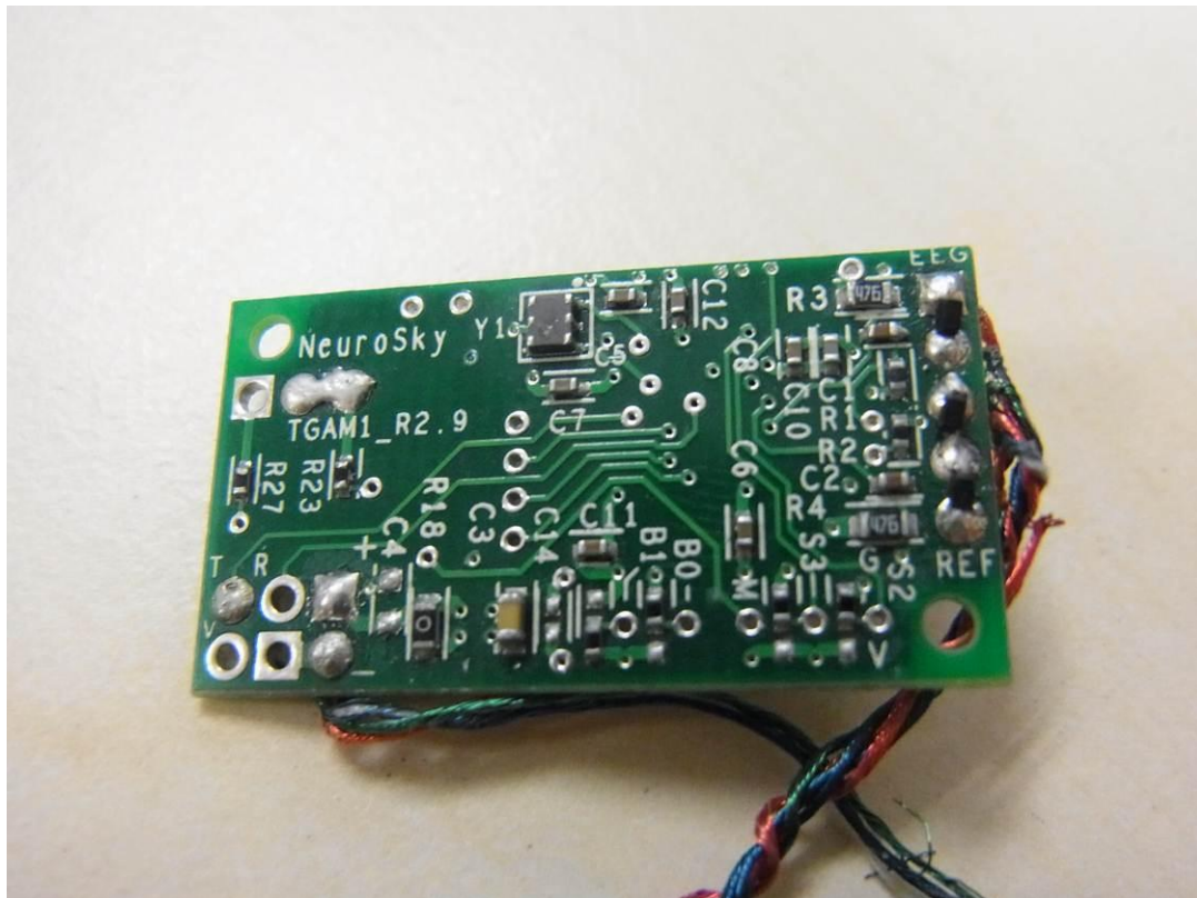
Fig. 4: Internal view
