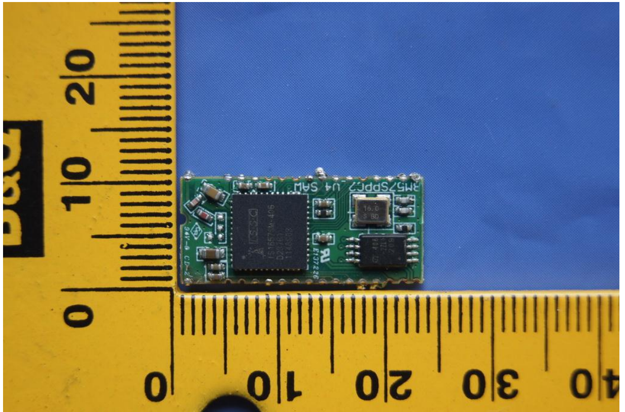
Fig. 7: Internal view
