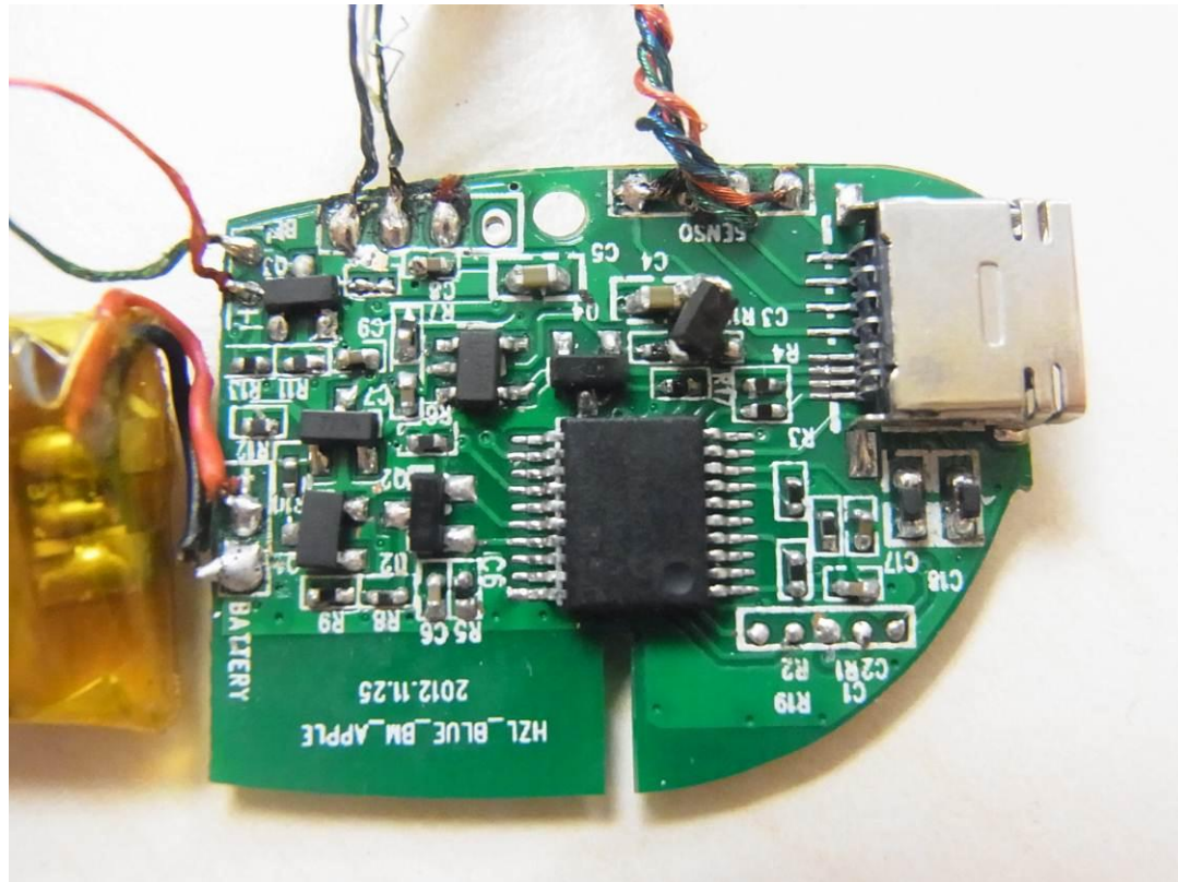
Fig. 5: Internal view
