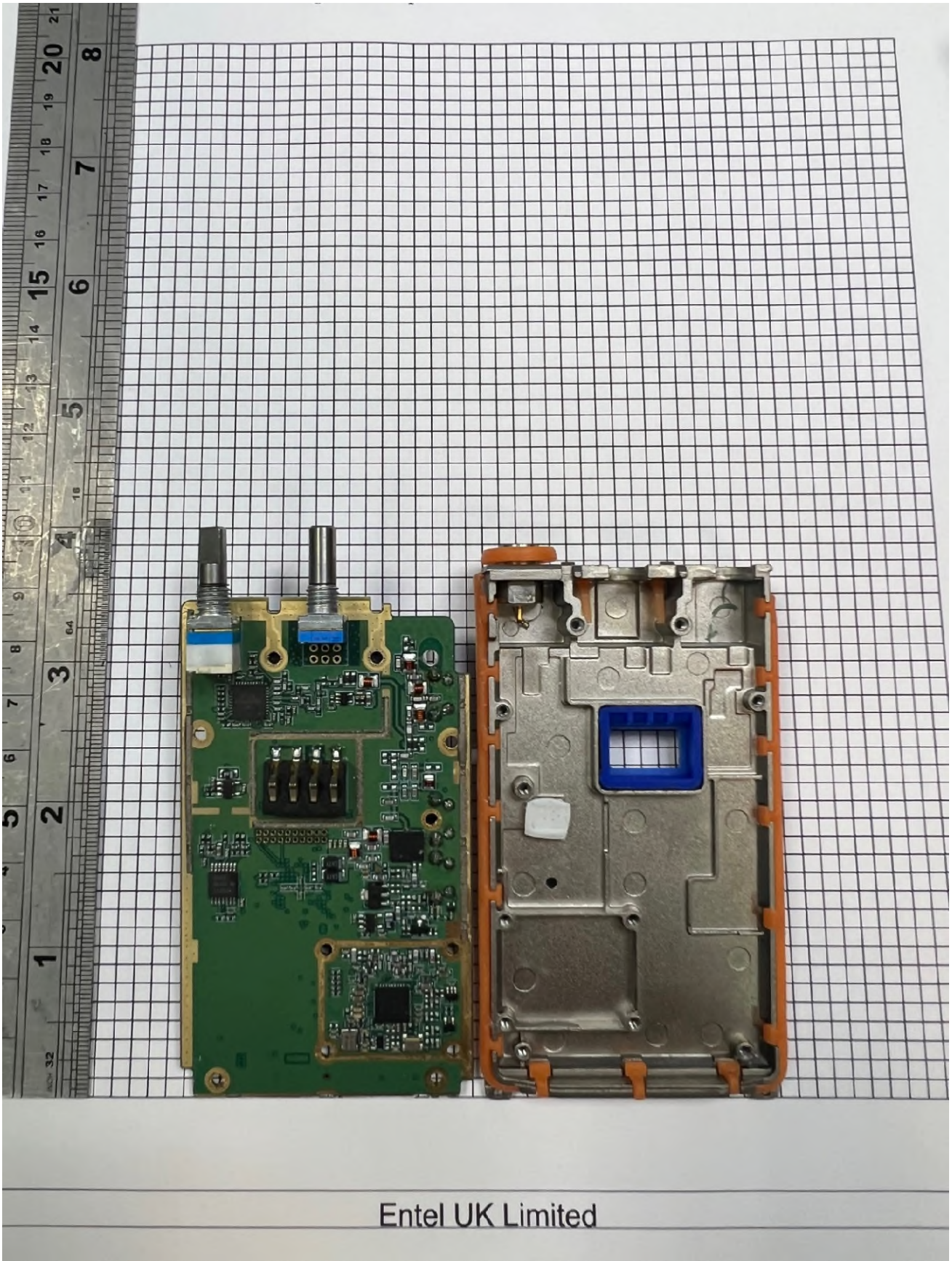
Main board bottom with chassis
