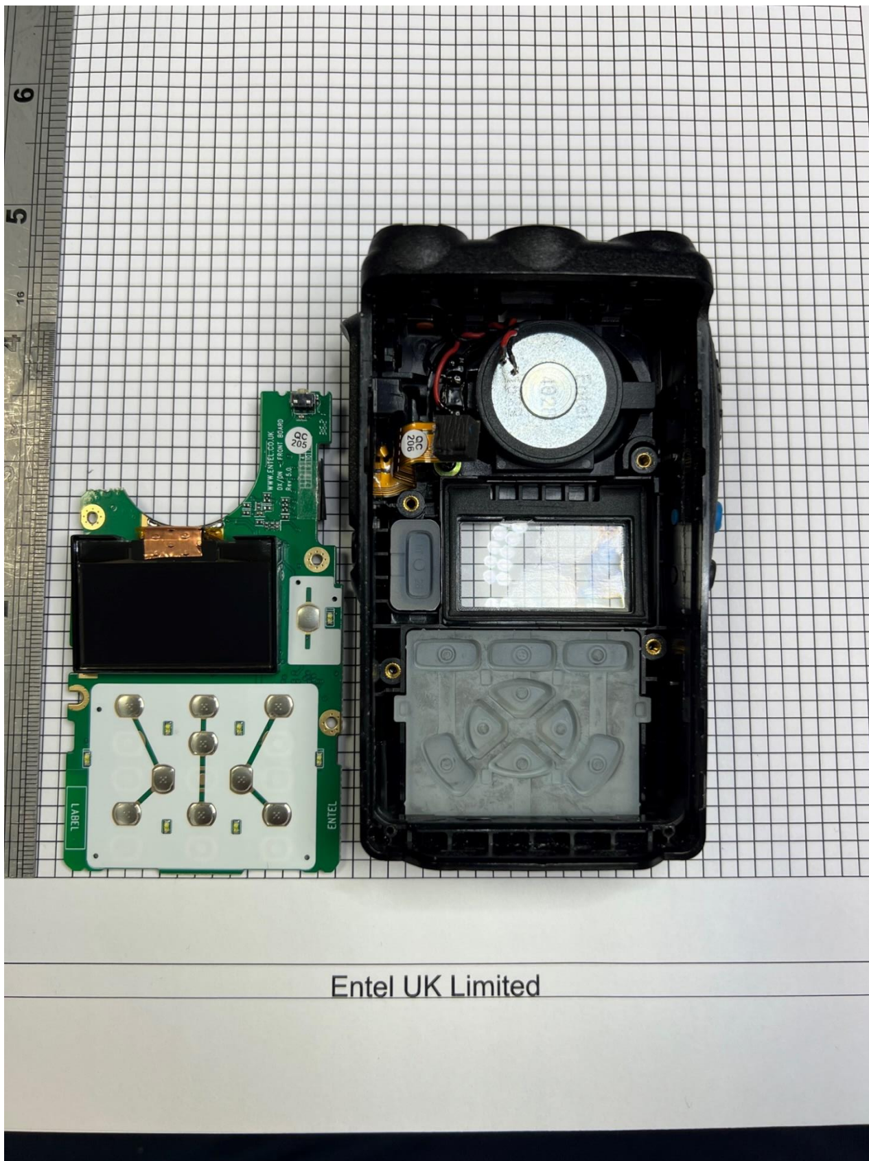
Front board bottom with cabinet
