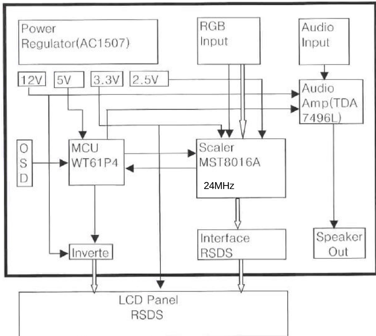
SDM-1503A BLOCK DIAGRAM
