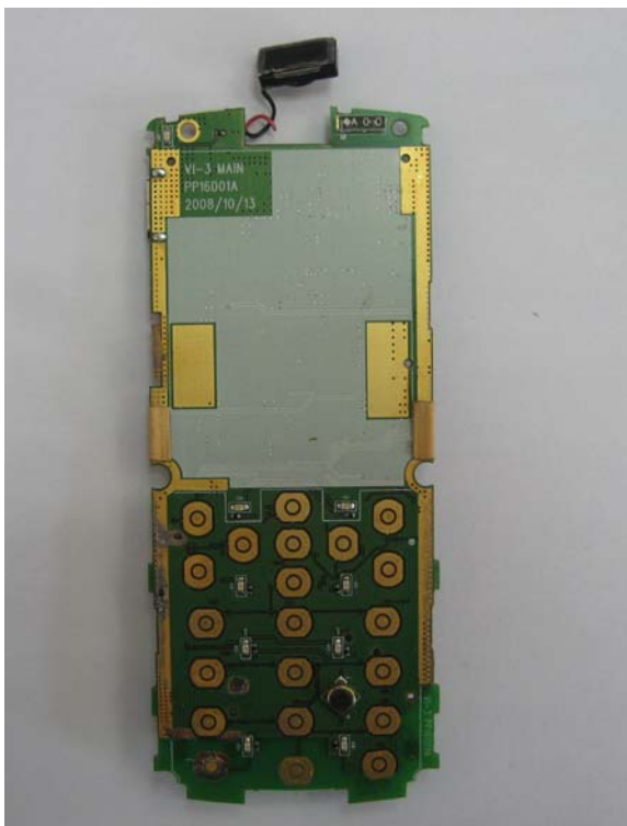
Picture 2: The top view of the PCB with the shielding cover removed
