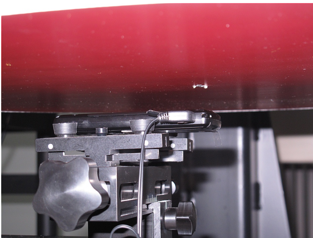
Picture 8: Body SAR Back to the phantom with earphone
