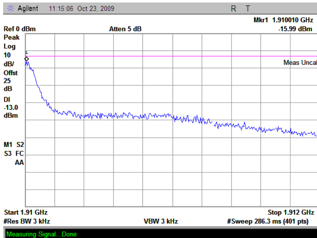
(Plot B: Channel = 810)
