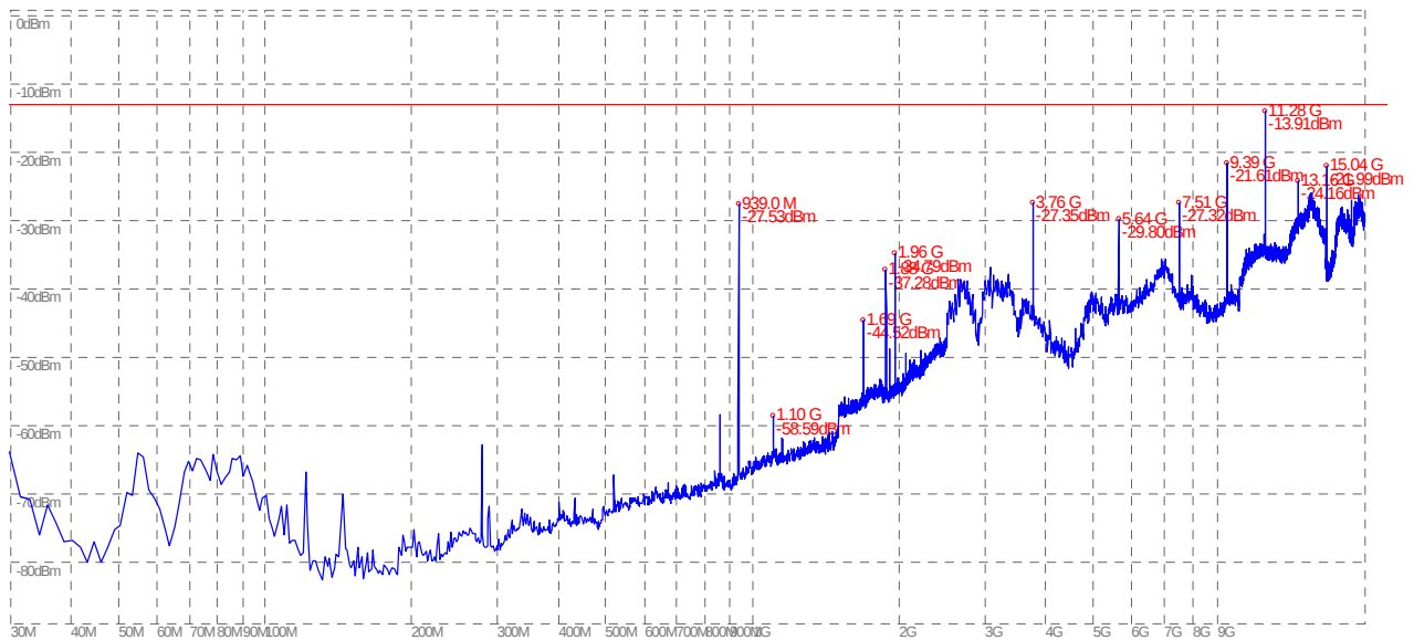
(Plot B.2: GSM 1900MHz Channel = 661, Test Antenna Vertical)
