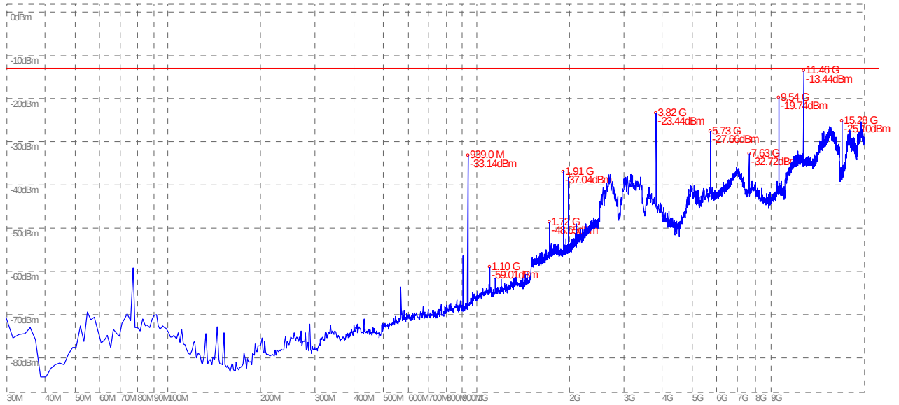
(Plot C.1: GSM 1900MHz Channel = 810, Test Antenna Horizontal)
