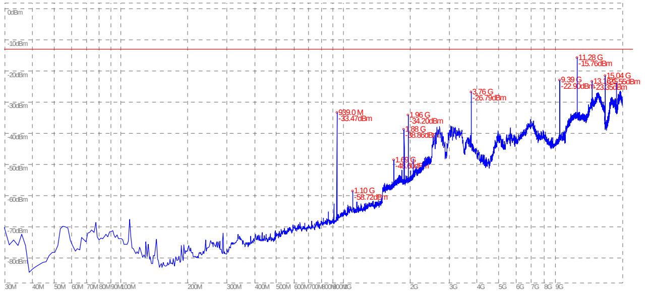
(Plot B.1: GSM 1900MHz Channel = 661, Test Antenna Horizontal)
