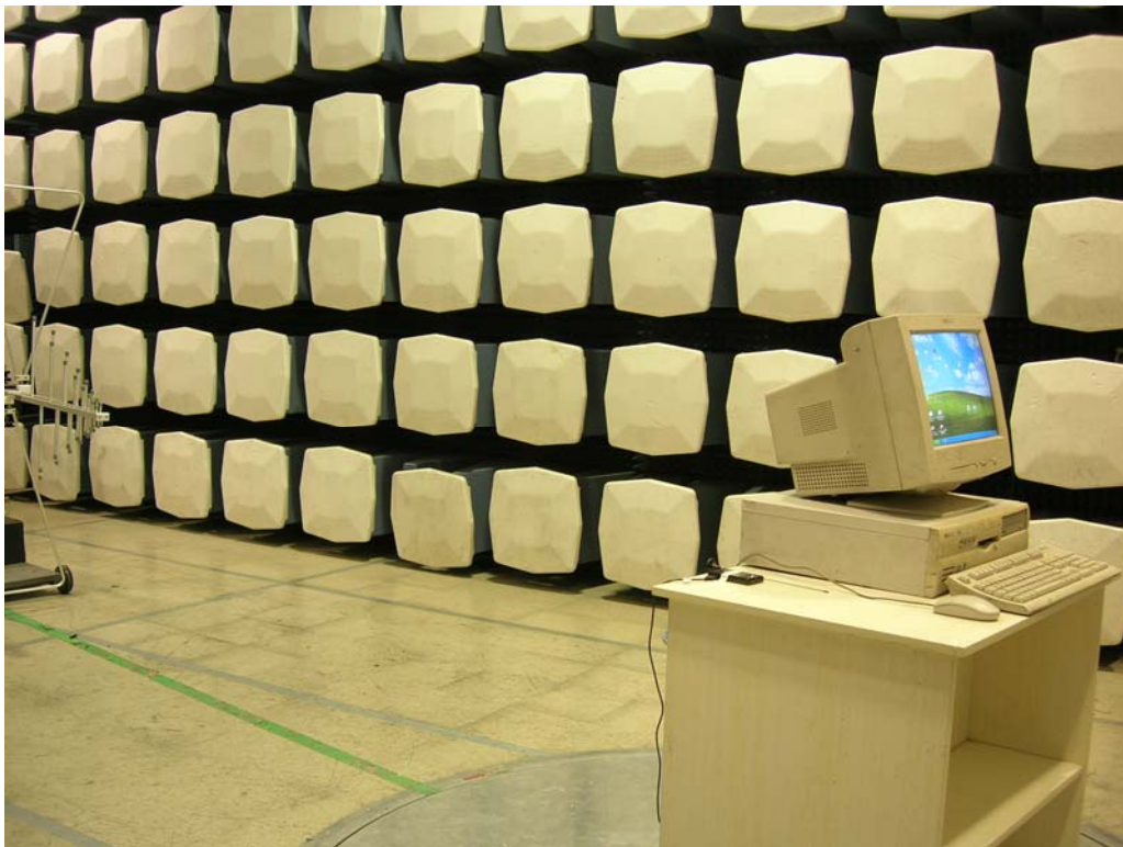
Figure RE: Test Setup face
