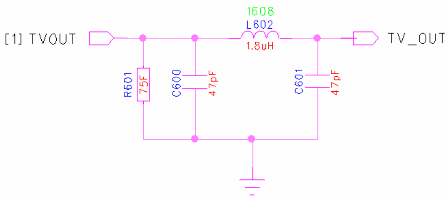
Figure 28. TV out Matching Circuit.
