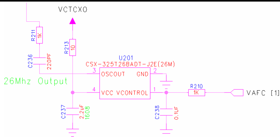
Figure 37. The AFC and VCTCXO Circiut diagram
