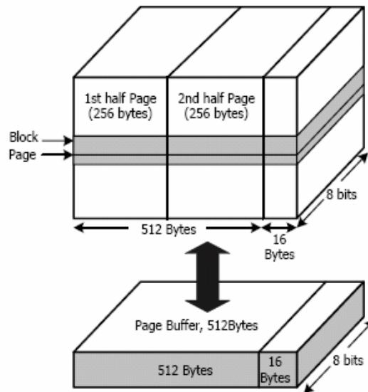
Figure 1. Memory Array Organization
