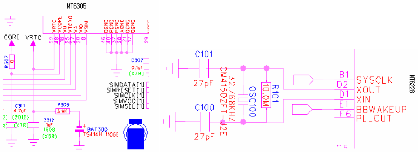
Figure 19. RTC Circuit
