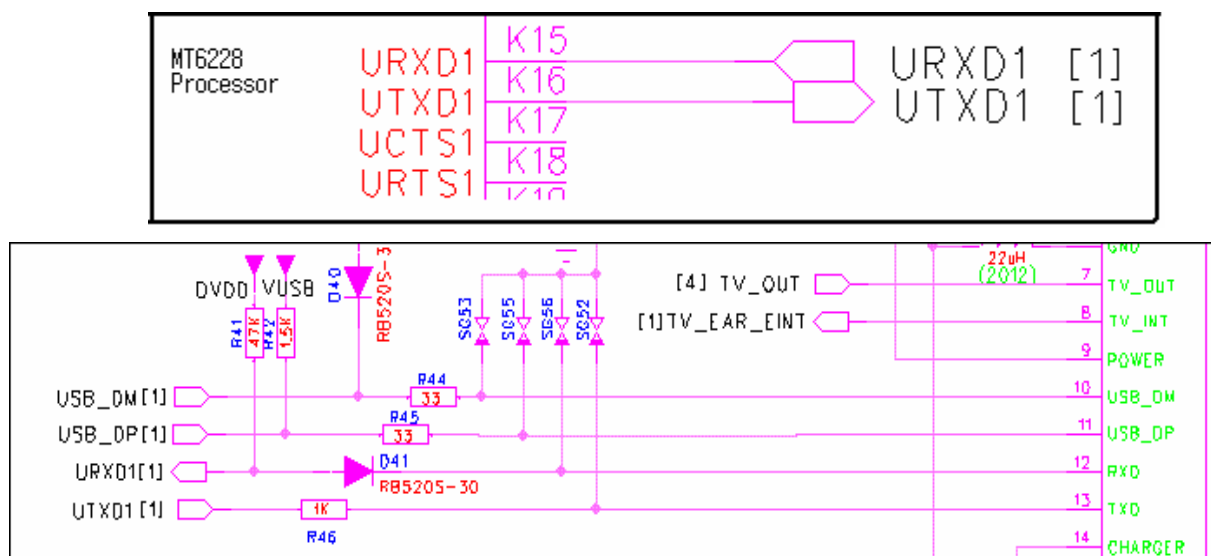
Figure 9. Circuit from MT6228 to I/O Connector
