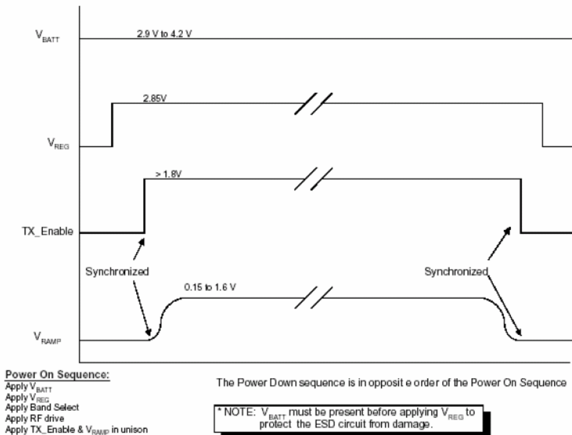
Figure 49. Power control sequence
