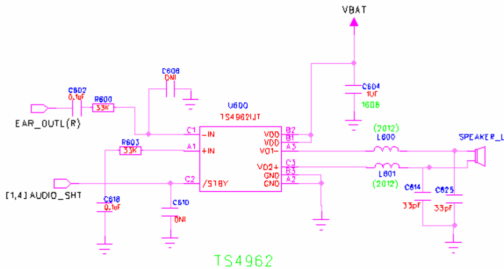
Figure 32. Audio Amp Circuit Diagram.
