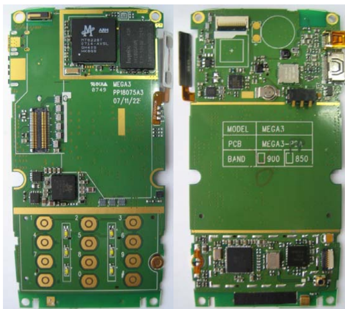
Picture 3: The sample with the shielding cover removed
