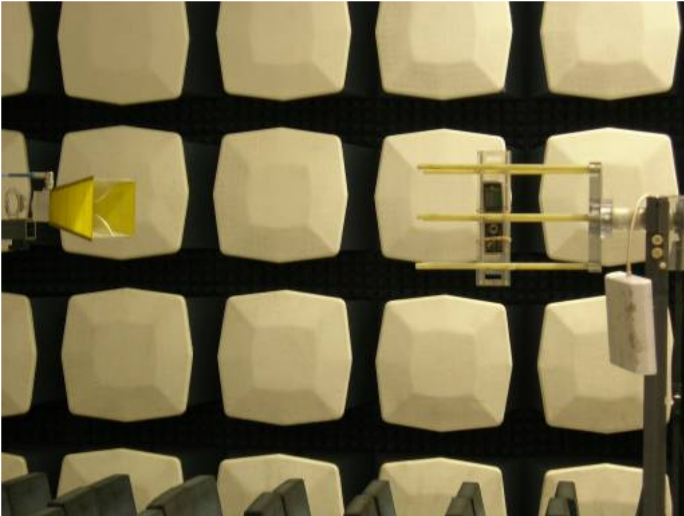
Picture 12: setup for Radiated Spurious Emission and ERP
