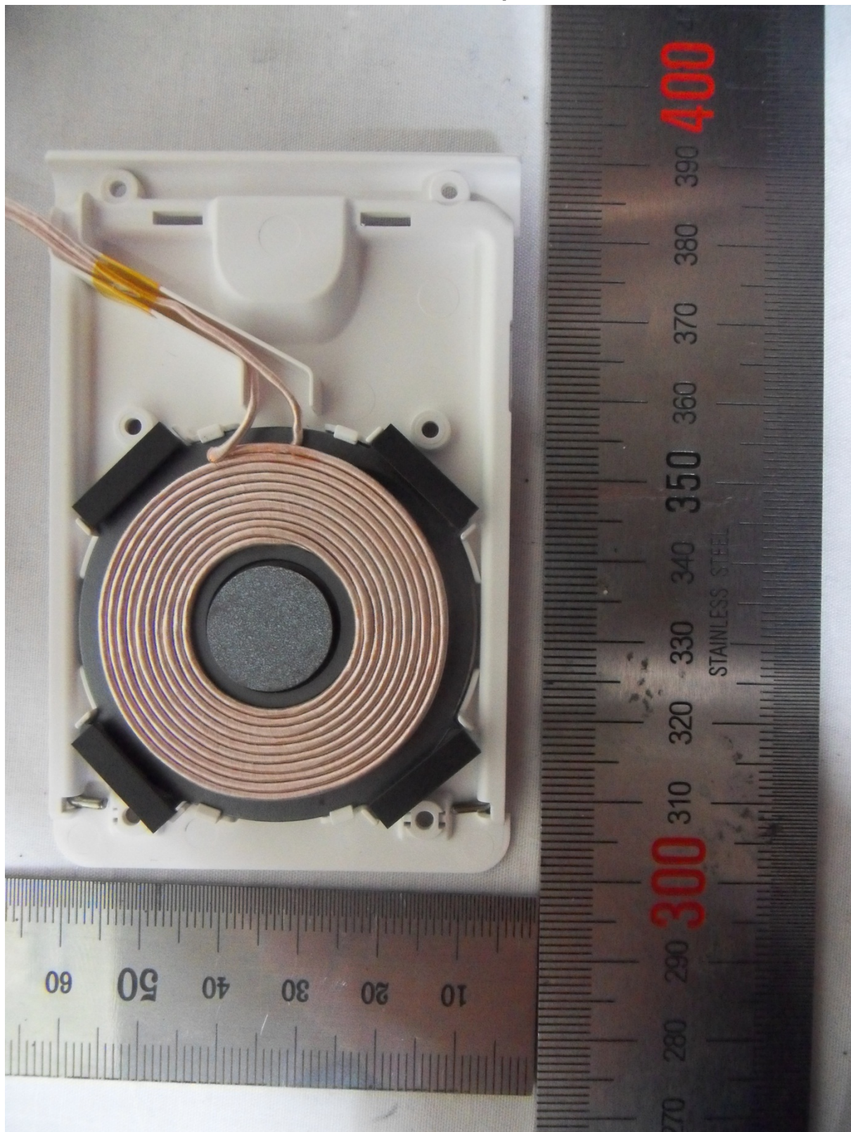
View of coil (Top)
