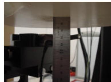
Fig. 19. Body SAR Test Setup with Holster
