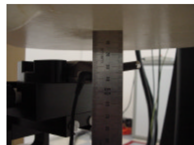
Fig. 19. Body SAR Test Setup with Holster
