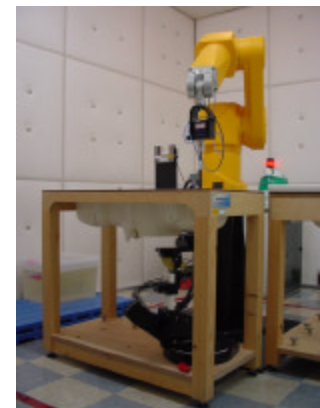
Figure 1. SAR System
