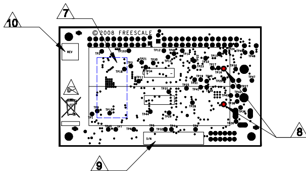
SECONDARY SIDE
