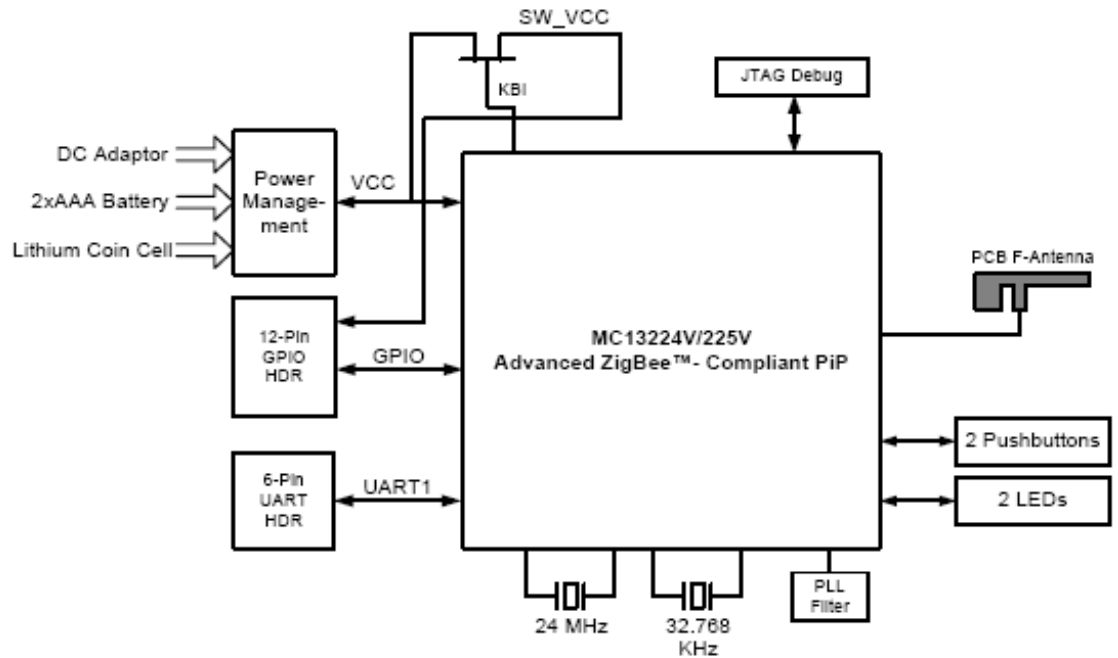
Figure 3-1. 1322x-LPB Block Diagram
