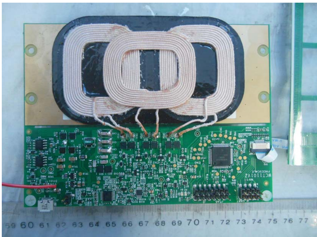
FIGURE 4 A28 MULTI-COIL WIRELESS CHARGER (M/N: WCT-5WTXMULTI) COIL
