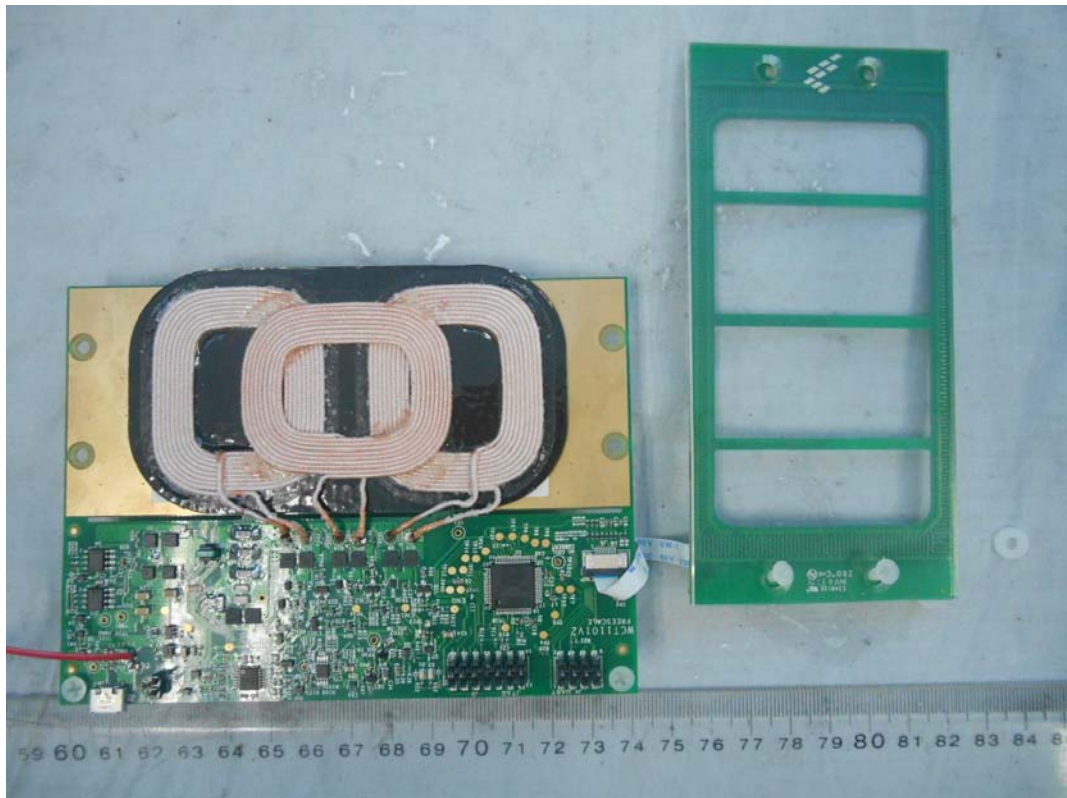
FIGURE 3 A28 MULTI-COIL WIRELESS CHARGER (M/N: WCT-5WTXMULTI) COVER REMOVED
