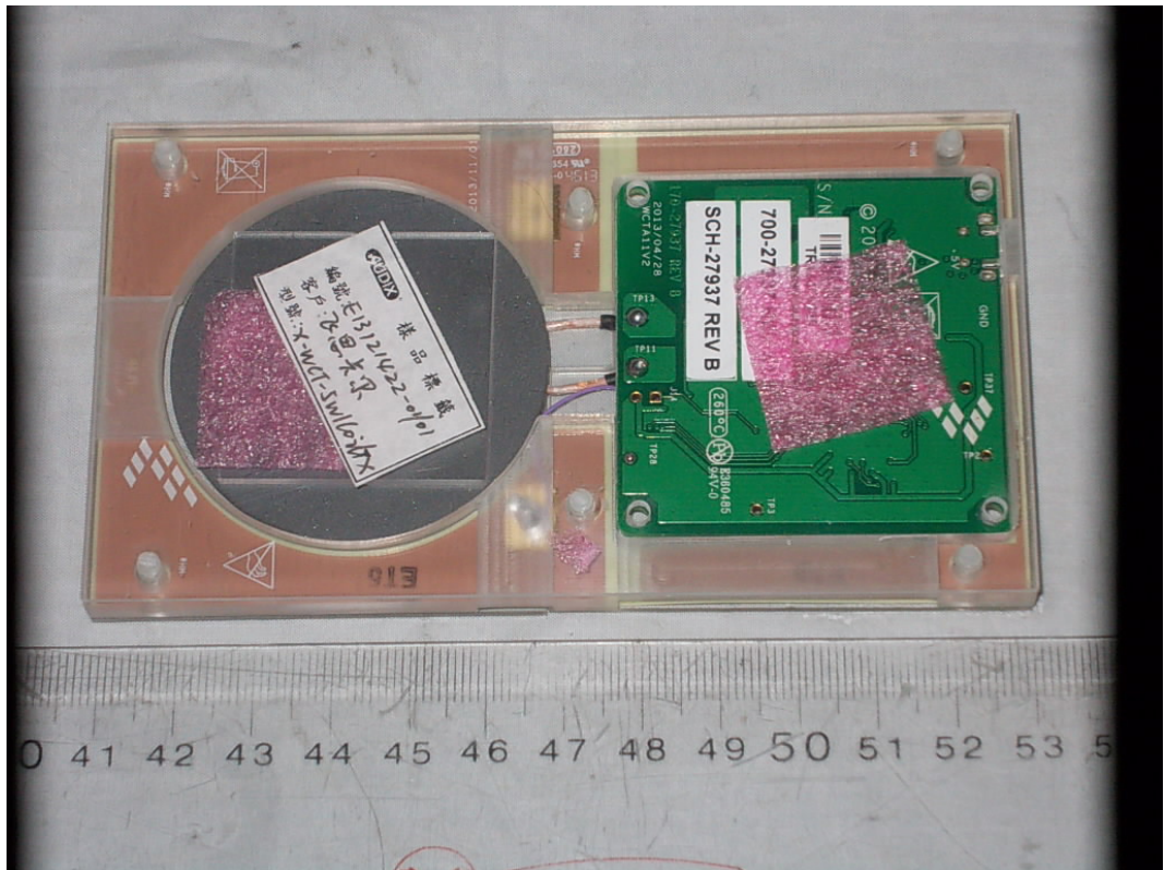
FIGURE 1 WIRELESS CHARGER TRANSMITTER (M/N: WCT-5W1COILT X ) GENERAL APPEARANCE (FRONT VIEW)
