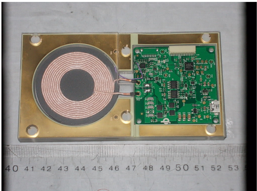
FIGURE 2 WIRELESS CHARGER TRANSMITTER (M/N: WCT-5W1COILT X ) GENERAL APPEARANCE (BACK VIEW)
