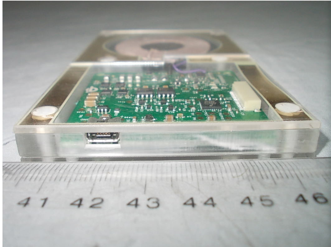
FIGURE 3 WIRELESS CHARGER TRANSMITTER (M/N: WCT-5W1COILTX) PORT VIEW
