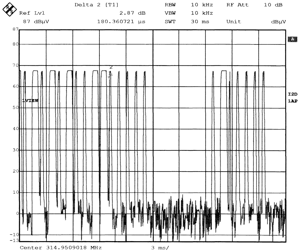
Figure C [Short Pulse]
