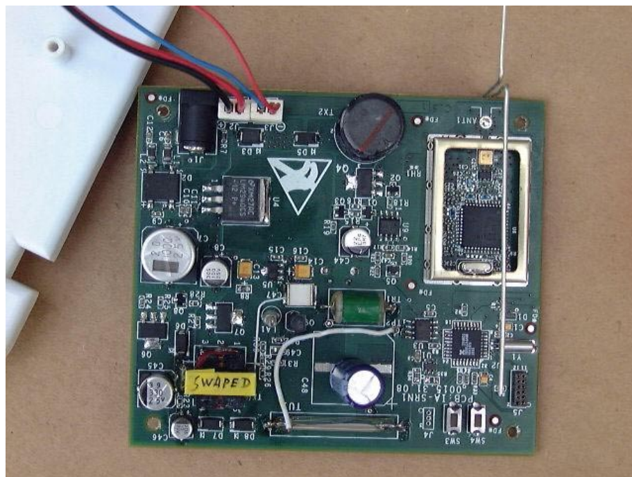
Figure 4 PCB Side 1 Without Shield
