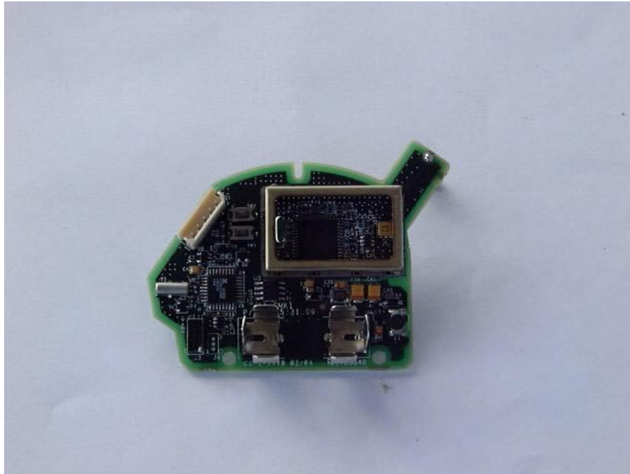
Figure 5 PCB Side 1 Without Shield
