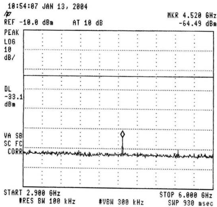
Figure 23.— 903.5 MHz
