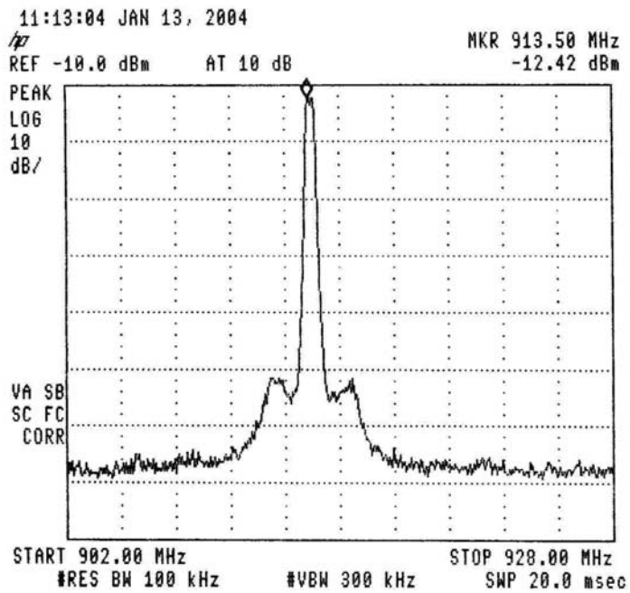
Figure 25.— 913.5 MHz
