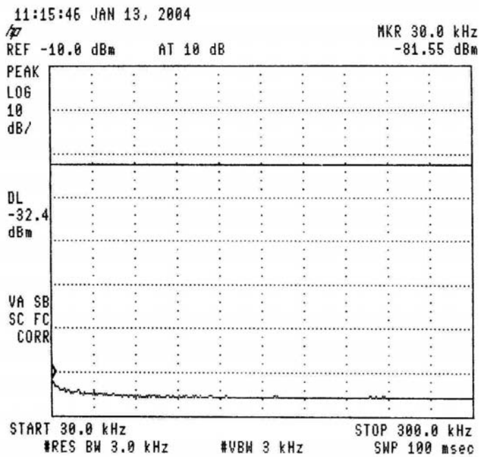
Figure 26.— 913.5 MHz
