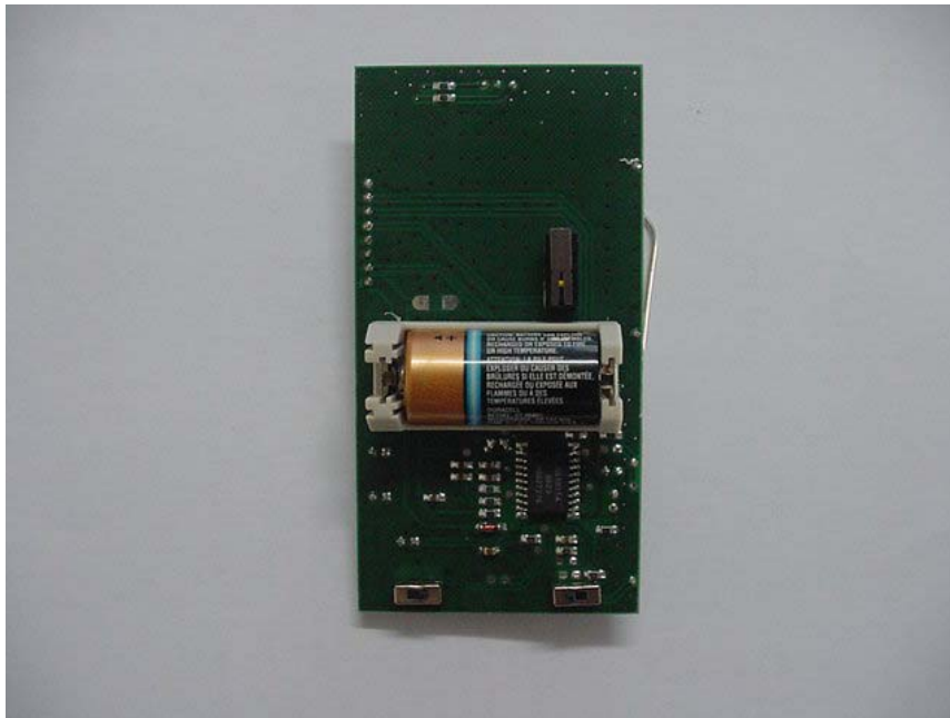
Figure 53 PCB Side 2
