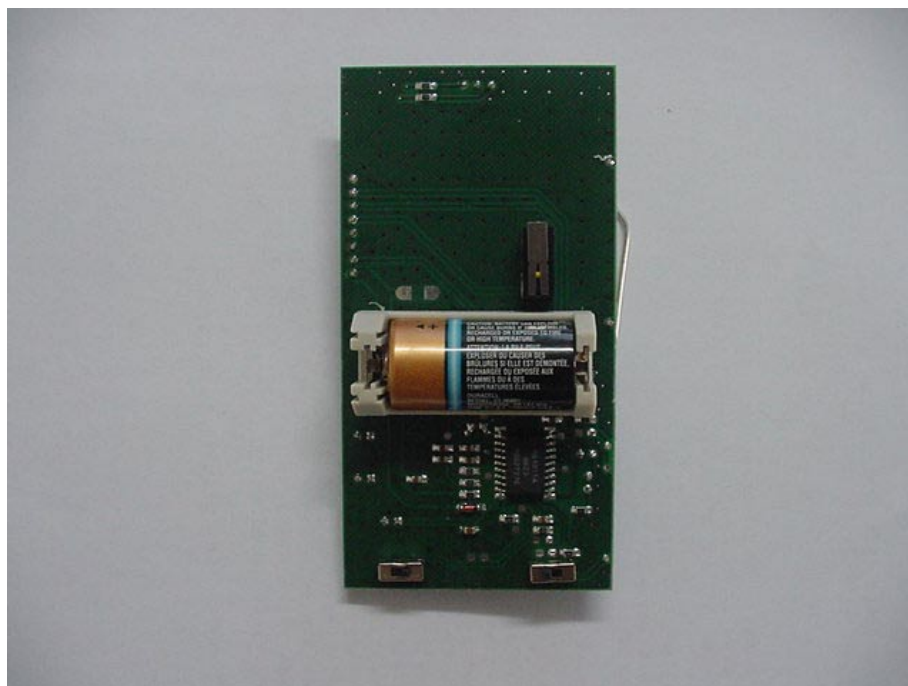
Figure 6 PCB Side 2
