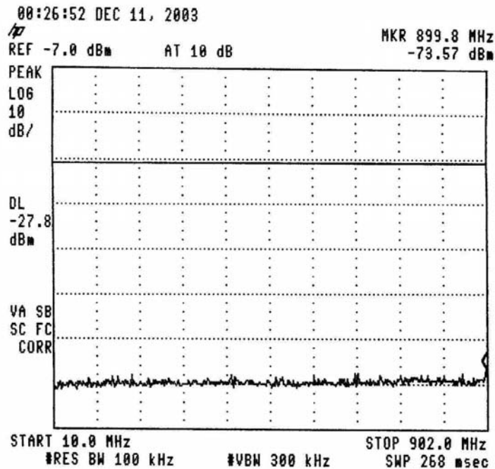
Figure 28.— 913.5 MHz
