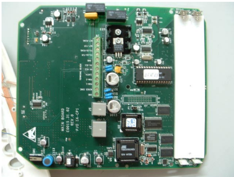
Figure 2 PCB 1 Side 1 Without Batteries
