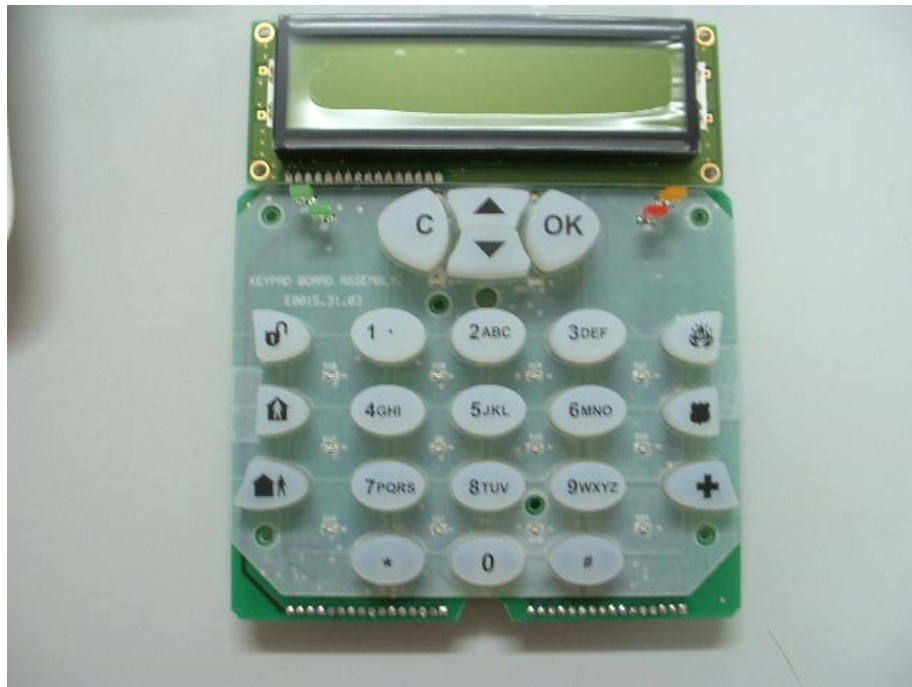
Figure 7 PCB 2 Side 2 With Cover (Buttons)
