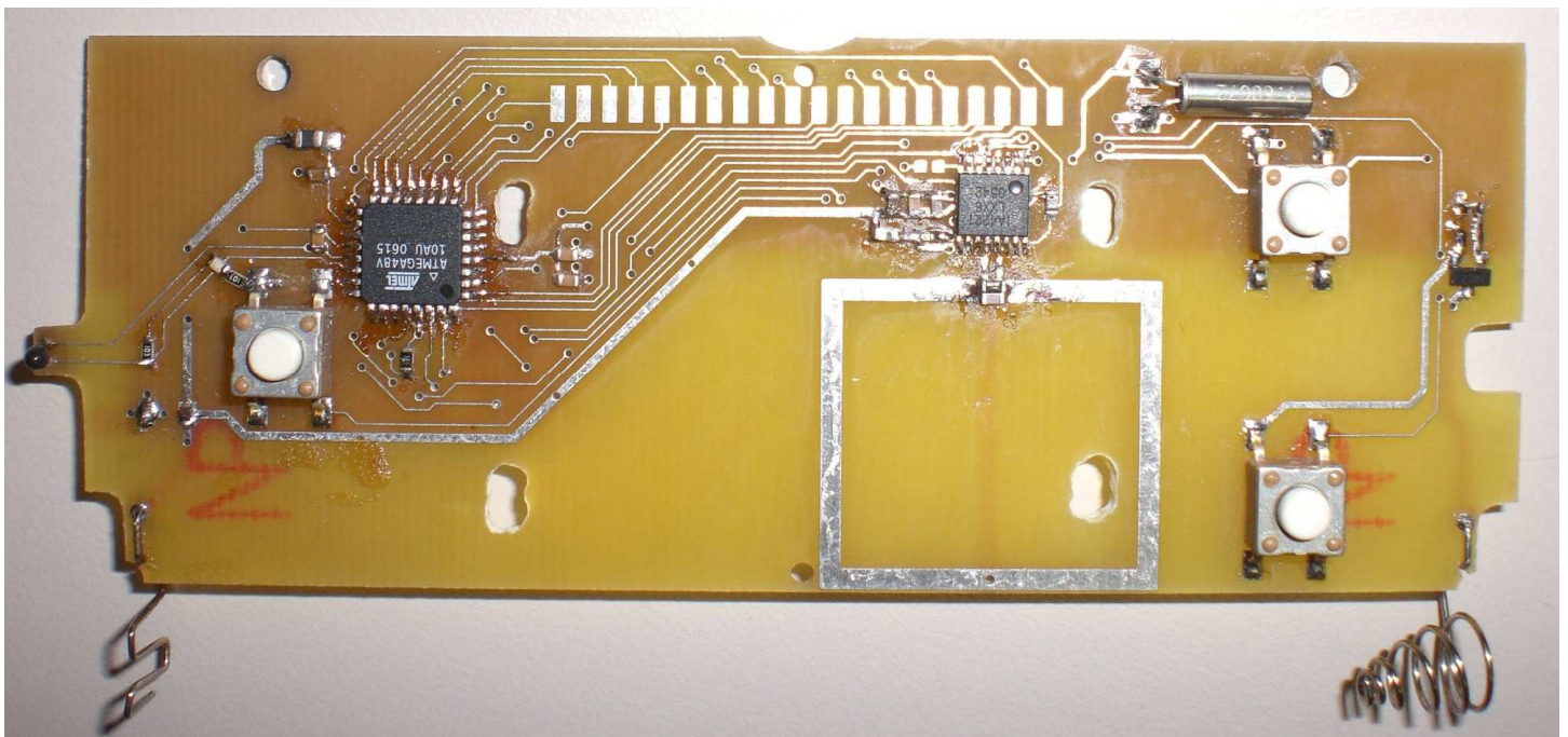
Component Side, LCD Removed
