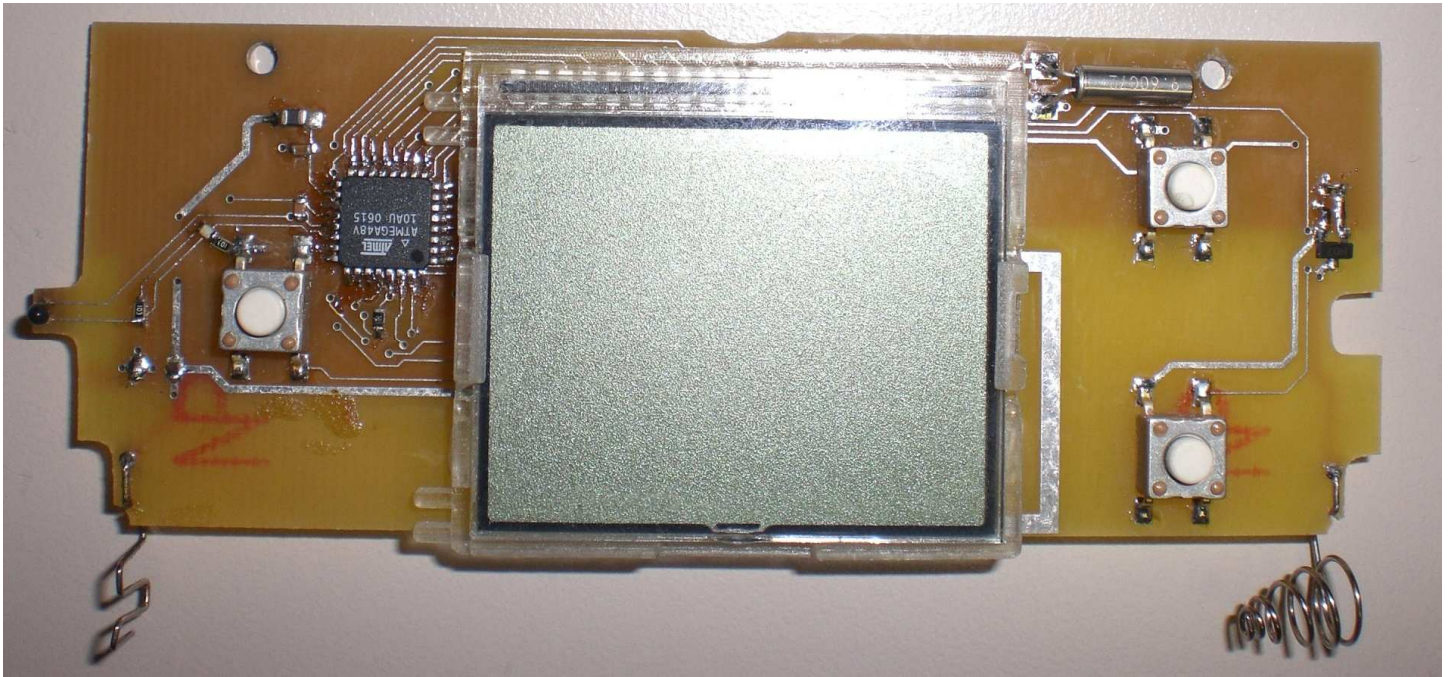
Component Side
