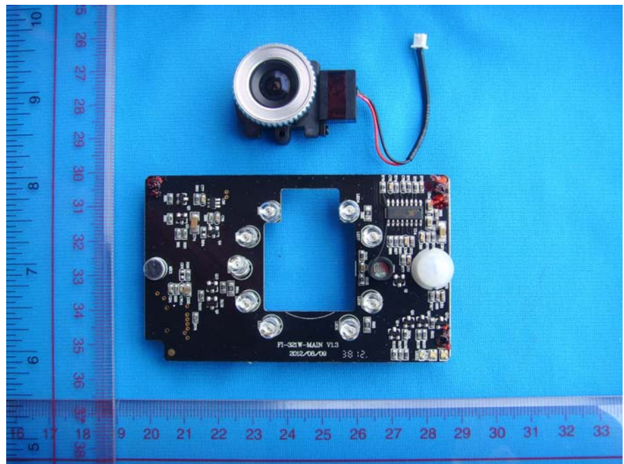
Details of: Infrared LED PCB and Lens
