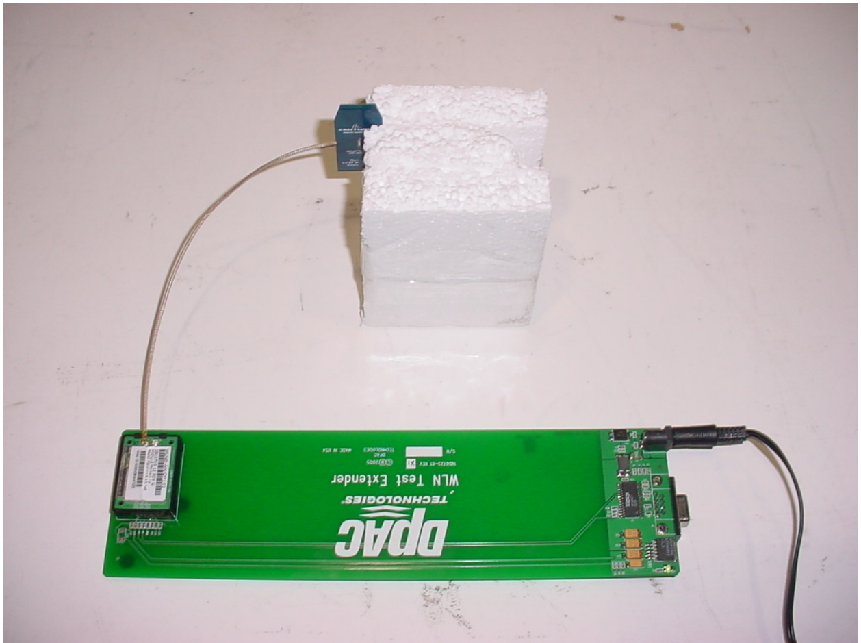
Figure 1: Test Setup – Centurion 1.5dBi Antenna – x Position
