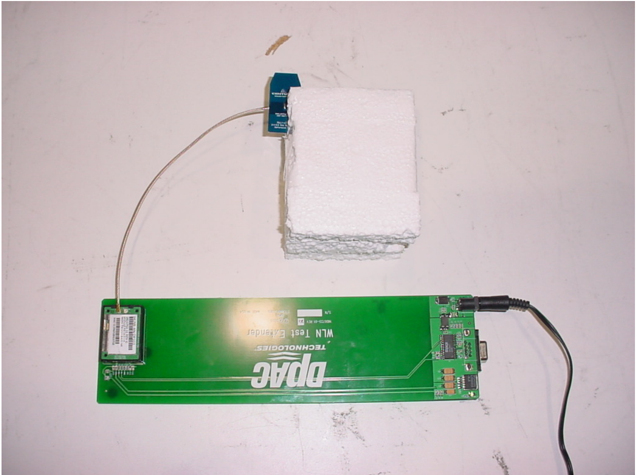
Figure 3: Test Setup – Centurion 1.5dBi Antenna – z Position
