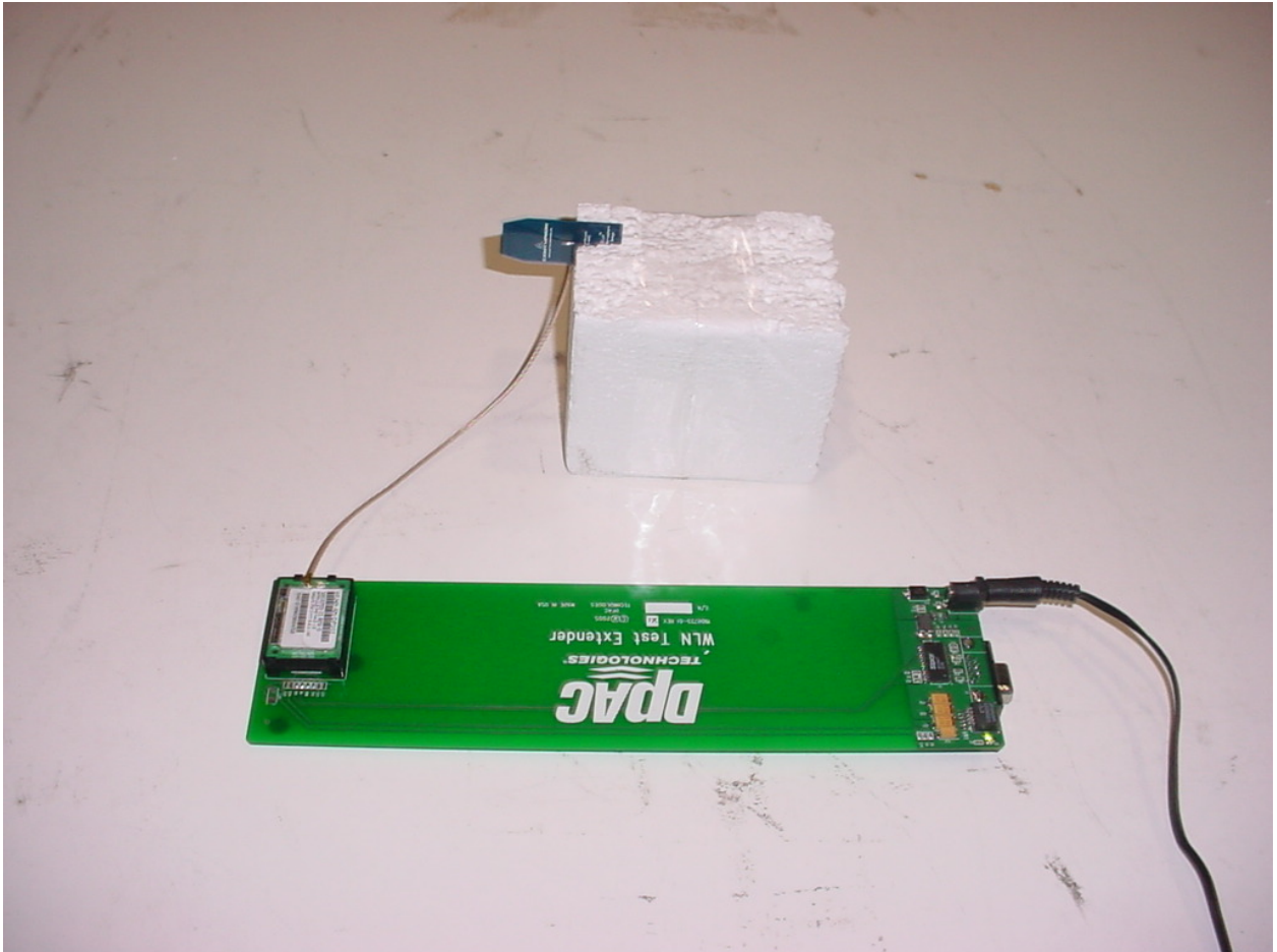
Figure 2: Test Setup – Centurion 1.5dBi Antenna – y Position
