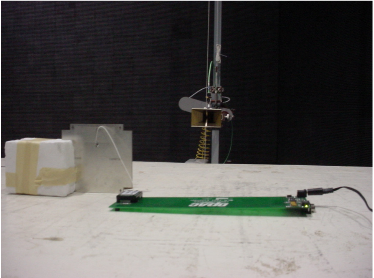
Figure 4: Test Setup – Cirronet 12dBi Patch Antenna
