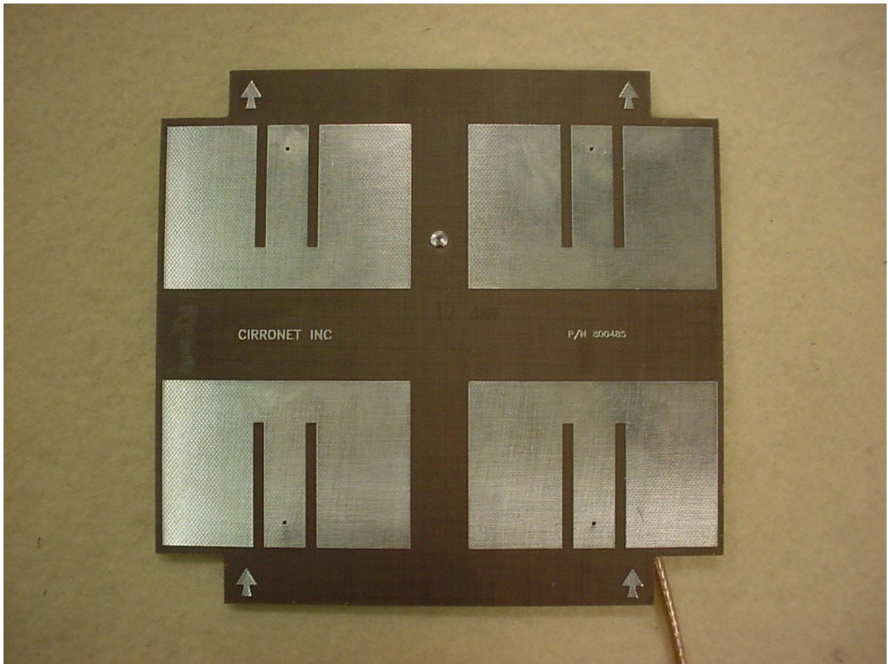
Figure 1: External – Cirronet 12dBi Antenna - Front
