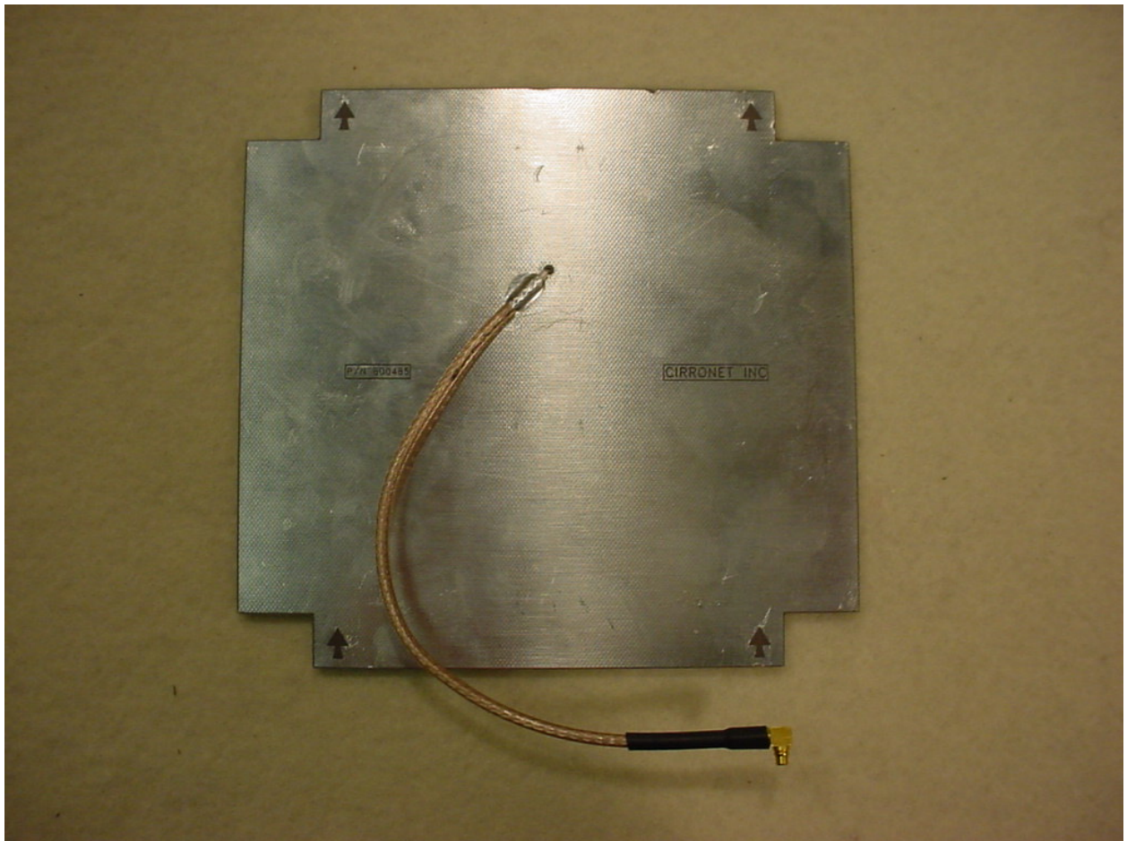
Figure 2: External – Cirronet 12dBi Antenna – Back
