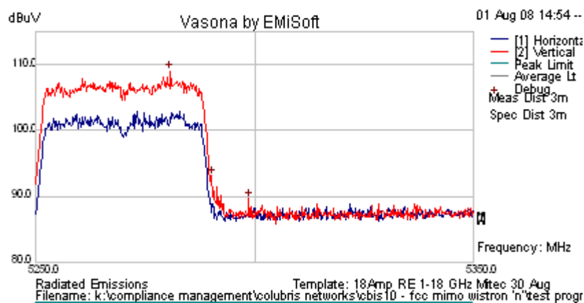
802.11a HT-40 – 5,270 MHz - External Antenna Lower Band Edge Peak Emission = 109.06 dBuV/m
