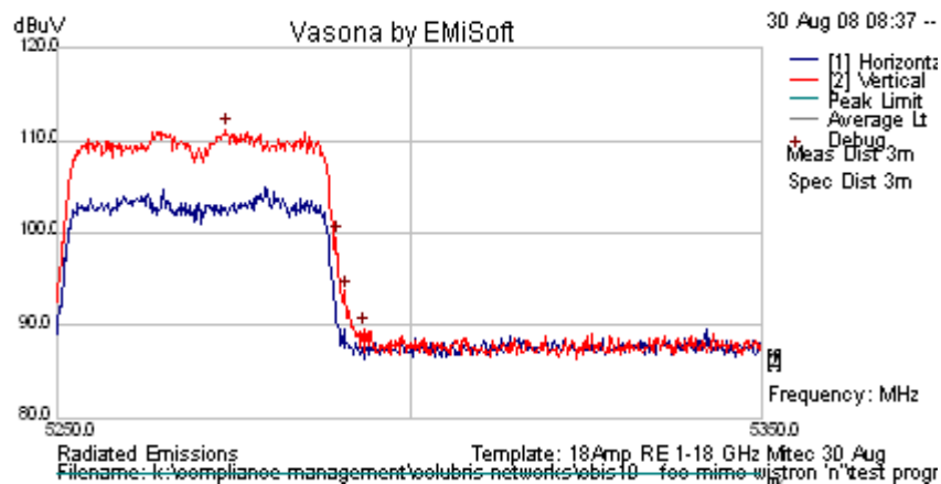
802.11a HT-40 – 5,270 MHz - Integral Antenna Lower Band Edge Peak Emission = 111.19 dBuV/m
