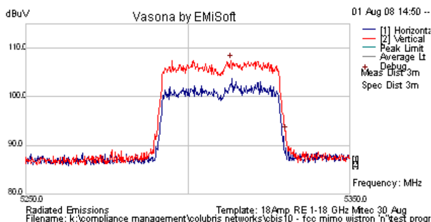
802.11a HT-40 – 5,310 MHz - External Antenna Lower Band Edge Peak Emission = 107.56 dBuV/m
