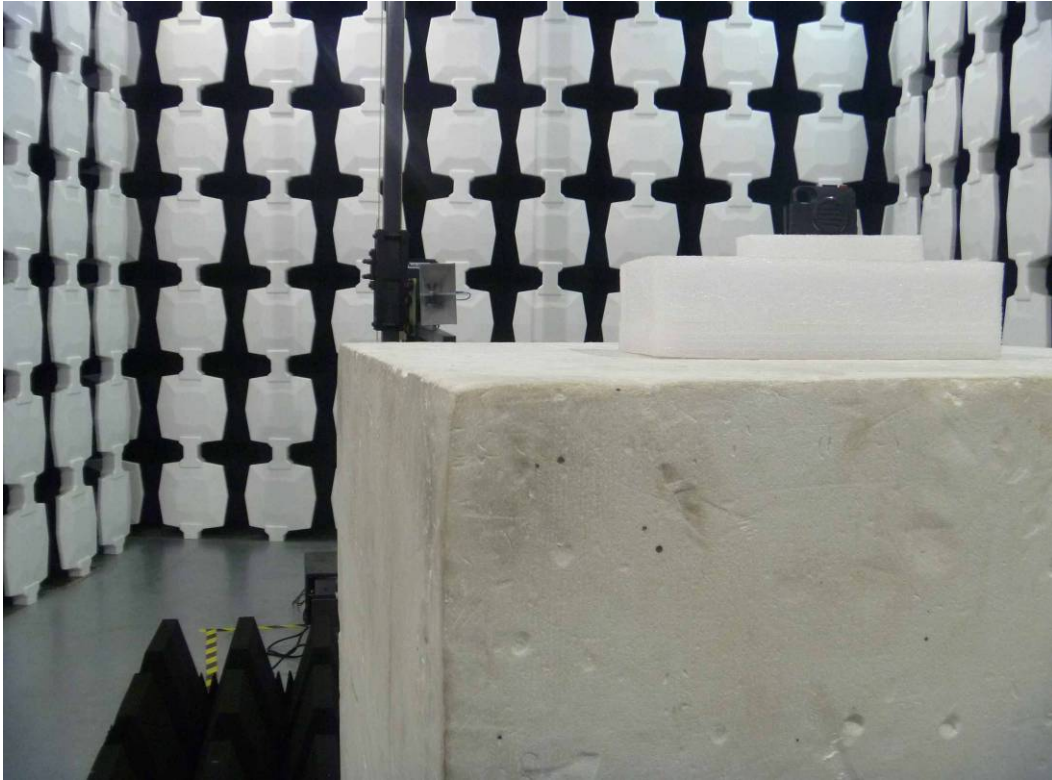
Description: Radiated Spurious Measurement Setup (Above 1GHz)
