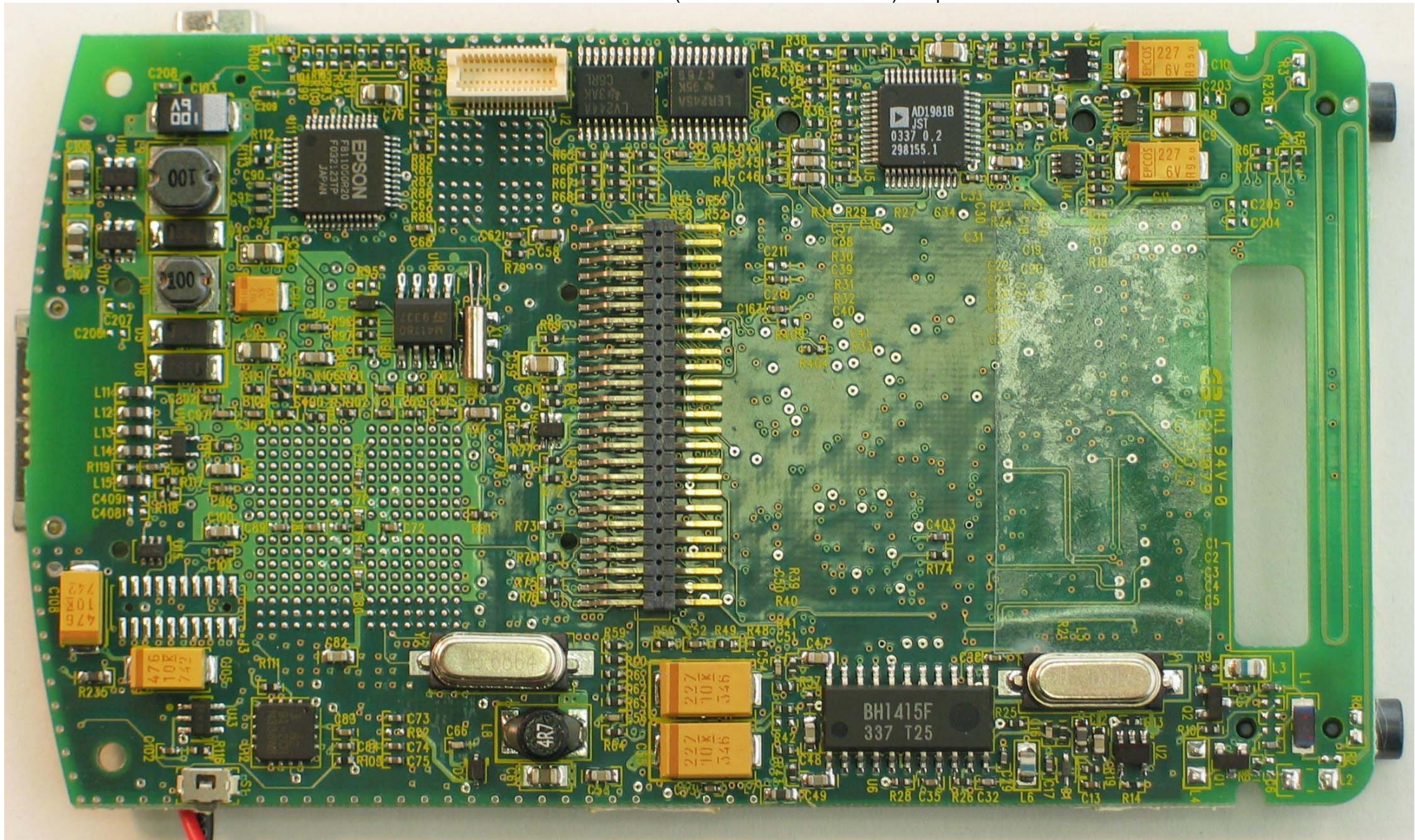
1000WF Internal - CPU PCB (with WIFI Board removed) - Top View
