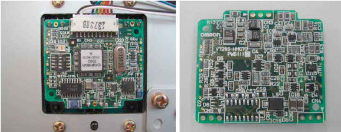
Photograph 6 & 7 – Top and Bottom View of the RFID Read/Write Control PCB
