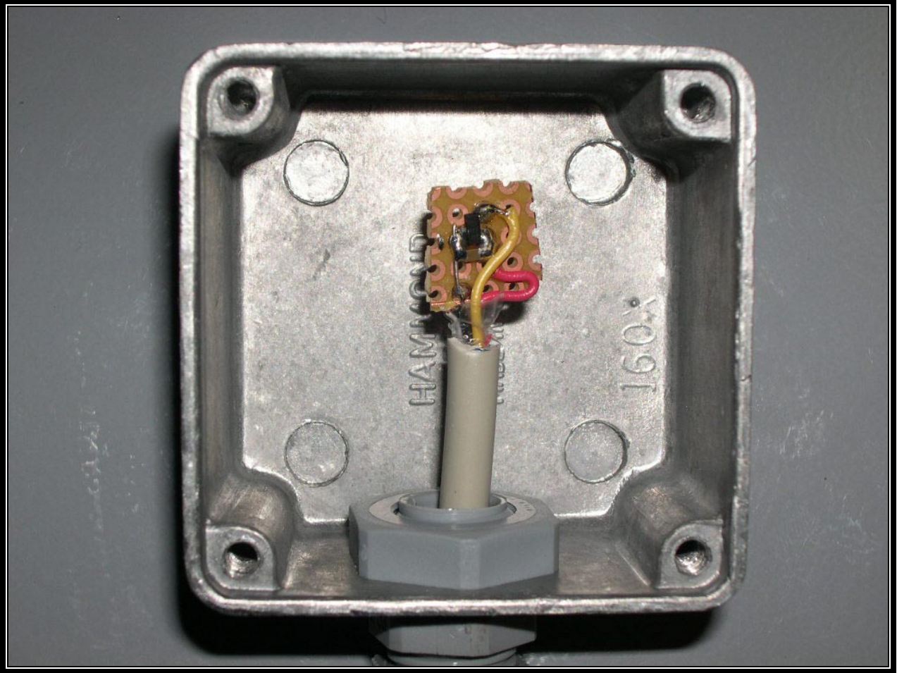
PHOTOGRAPH 44: SENSOR-TOP VIEW
