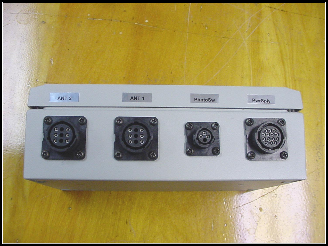
PHOTOGRAPH 14: ADU 2–FRONT VIEW
