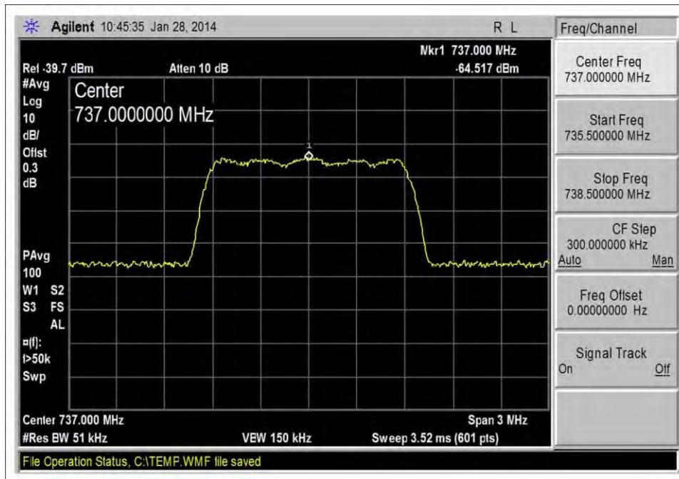
CDMA_DL 728-746_Input
