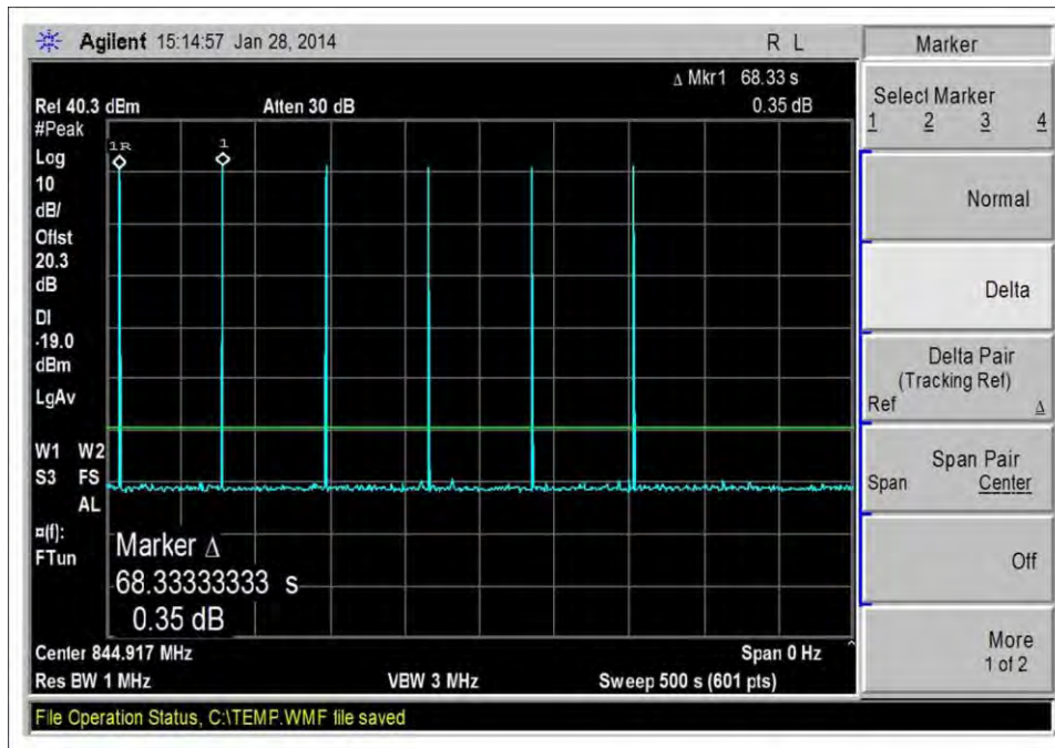
Oscillation Mitigation_UL_824-849MHz
