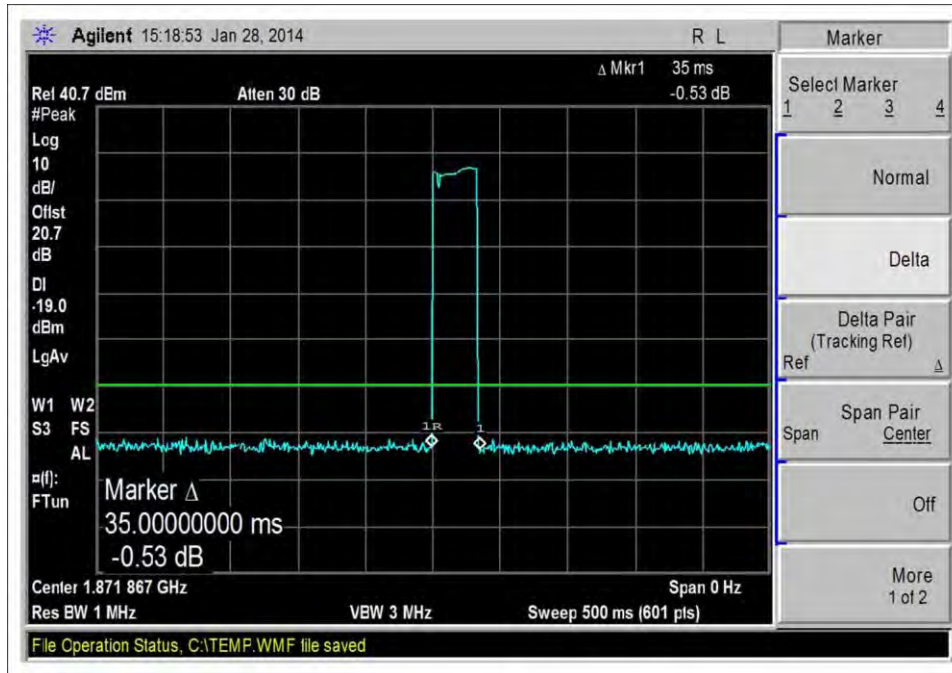
Oscillation Detection_UL_1850-1910MHz
