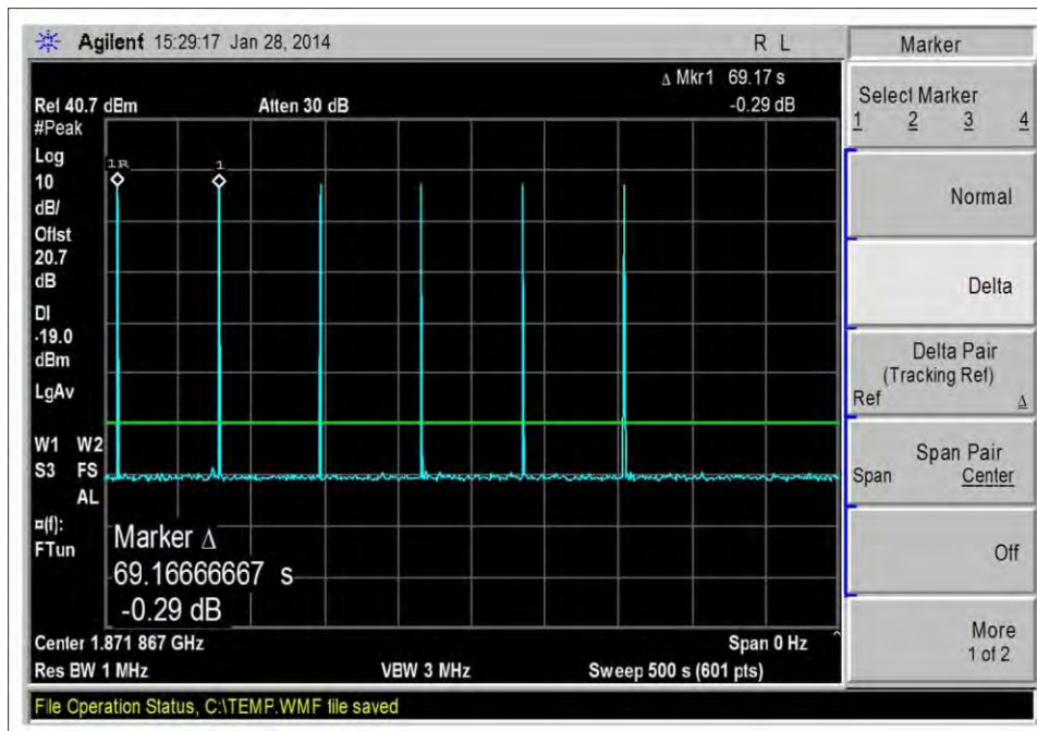
Oscillation Mitigation_UL_1850-1910MHz
