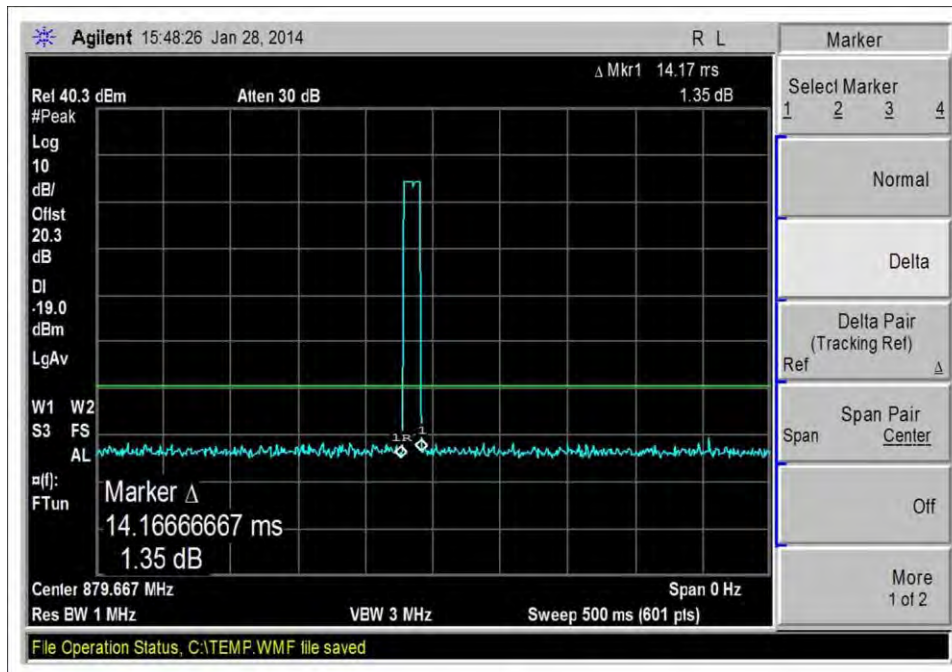
Oscillation Detection_DL_869-894MHz
