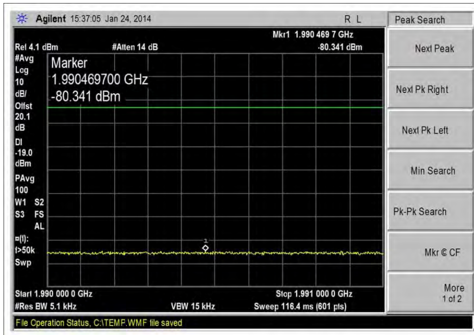
DL_1930-1990MHz_Hi CH_GSM_-20dbm
