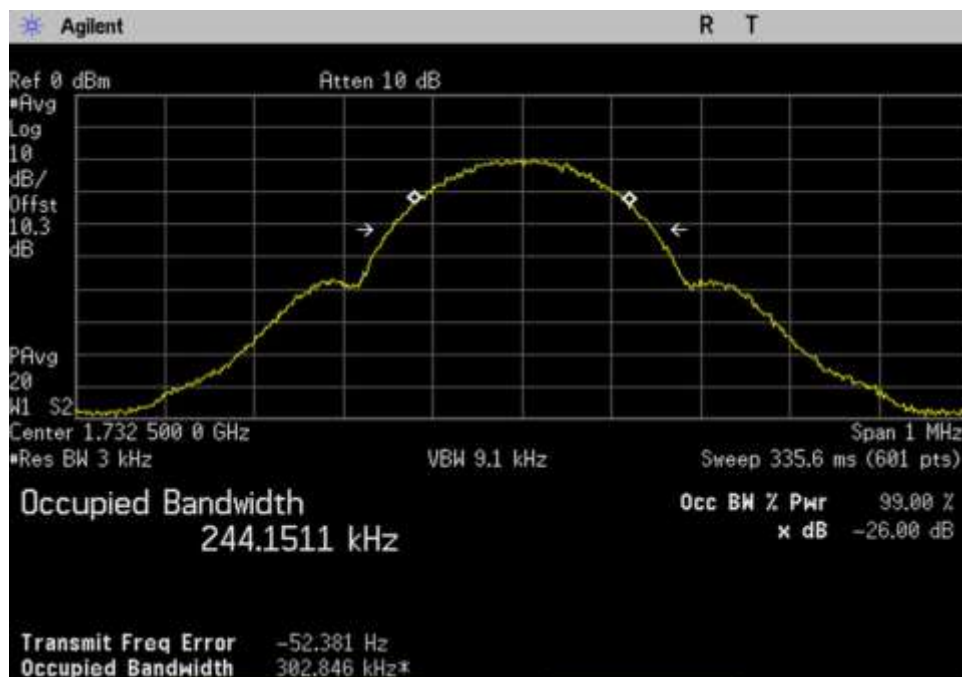
7.10 OBW-In_UL_1710-1755_GSM_1732.5MHz
