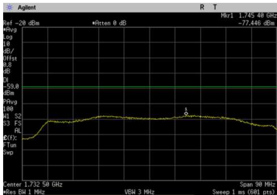
7.7 Noise_UL_1710-1755_ 1732.5MHz
