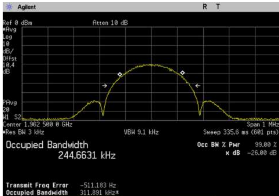
7.10 OBW-In_DL_1930-1995_EDGE_1962.5MHz
