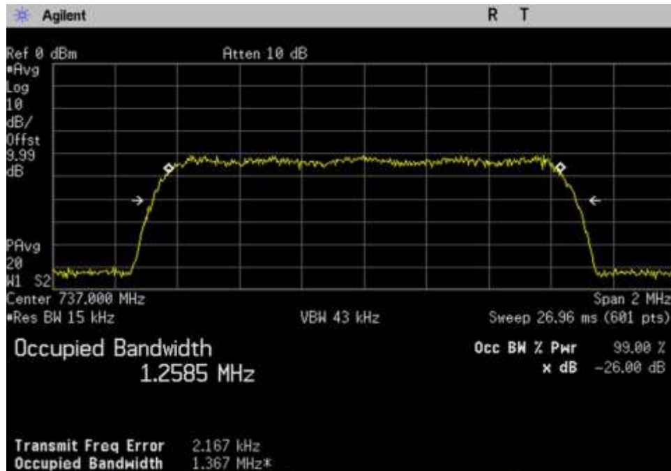
7.10 OBW-In_DL_728-746_CDMA_737MHz
