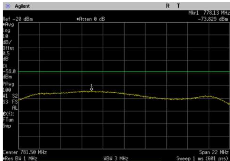
7.7 Noise_UL_776-787_ 781.5MHz
