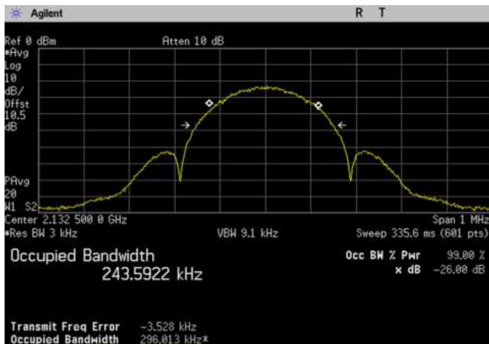
7.10 OBW-Out_DL_2110-2155_EDGE_ 2132.5MHz
