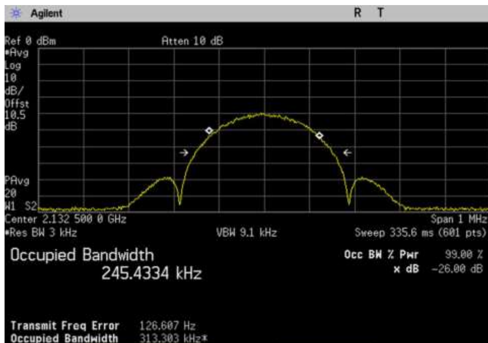
7.10 OBW-In_DL_2110-2155_EDGE_ 2132.5MHz
