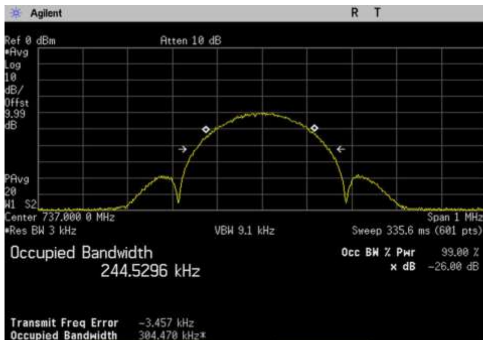
7.10 OBW-In_DL_728-746_EDGE_737MHz
