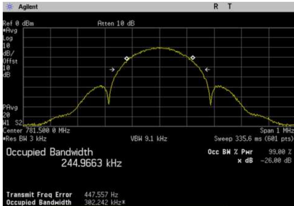
7.10 OBW-In_UL_776-787_EDGE_781.5MHz
