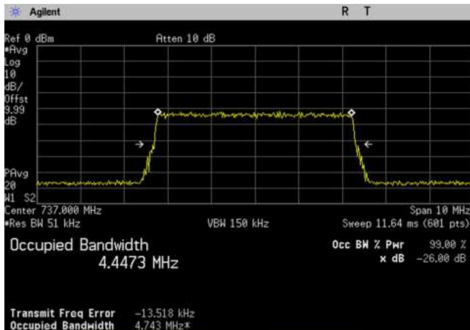
7.10 OBW-In_DL_728-746_LTE_737MHz
