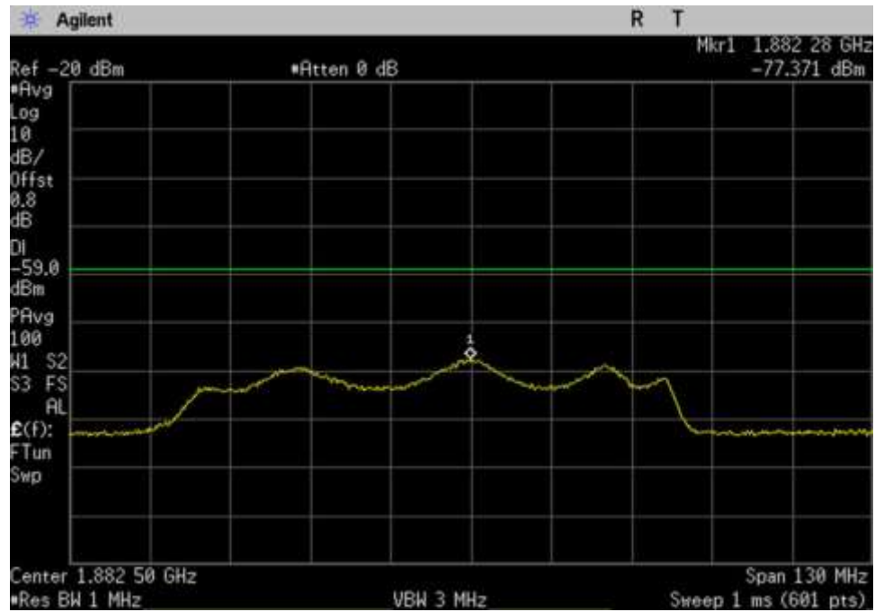
7.7 Noise_UL_1850-1915_ 1882.5MHz
