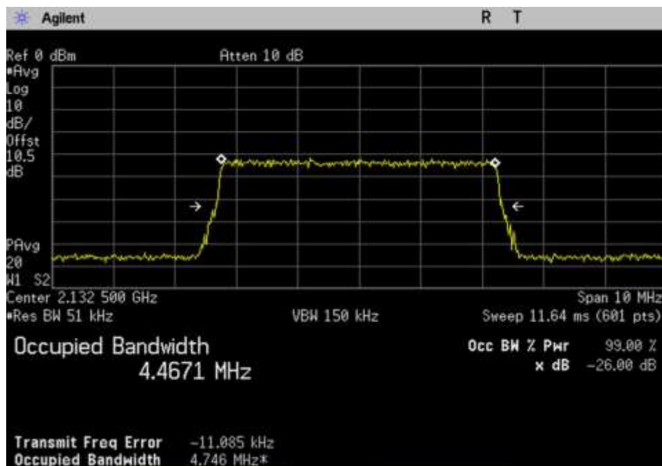
7.10 OBW-In_DL_2110-2155_LTE_ 2132.5MHz
