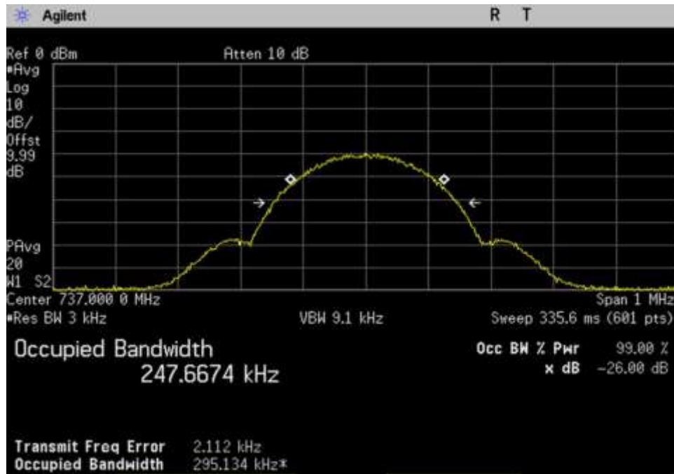
7.10 OBW-In_DL_728-746_GSM_737MHz
