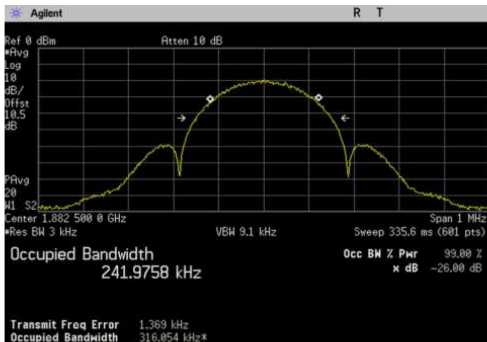
7.10 OBW-In_UL_1850-1915_EDGE_1882.5MHz
