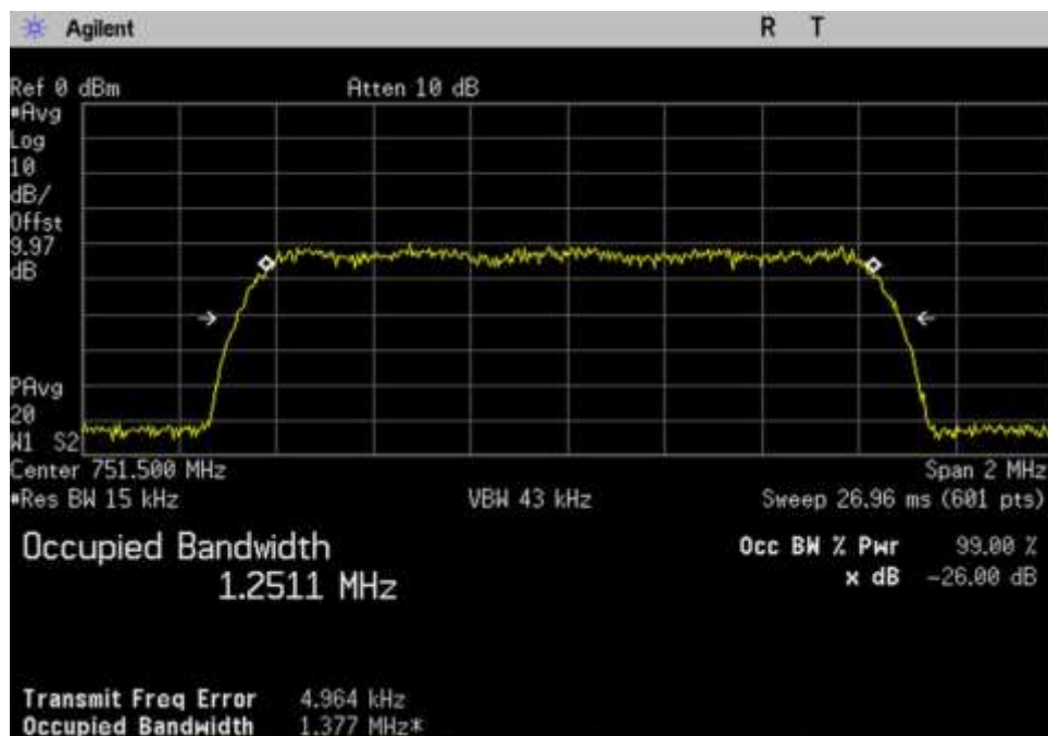
7.10 OBW-In_DL_746-757_CDMA_751.5MHz
