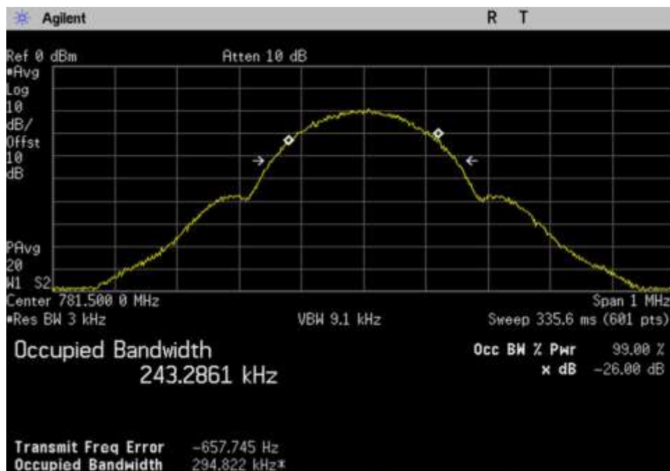
7.10 OBW-In_UL_776-787_GSM_781.5MHz
