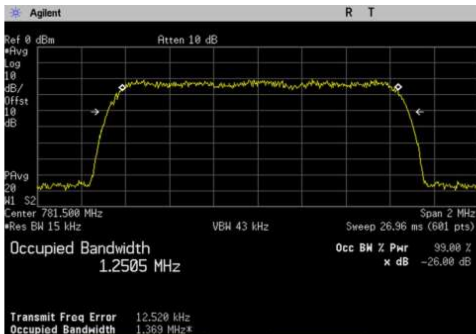
7.10 OBW-In_UL_776-787_CDMA_781.5MHz
