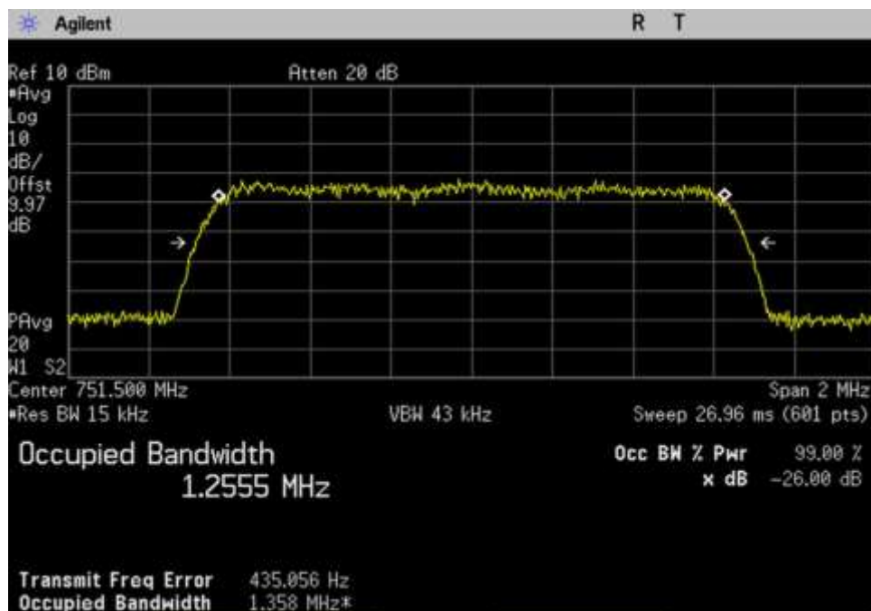
7.10 OBW-Out_DL_746-757_CDMA_751.5MHz
