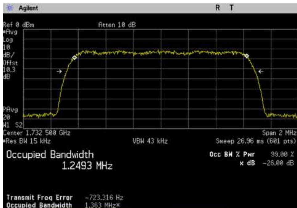
7.10 OBW-In_UL_1710-1755_CDMA_ 1732.5MHz
