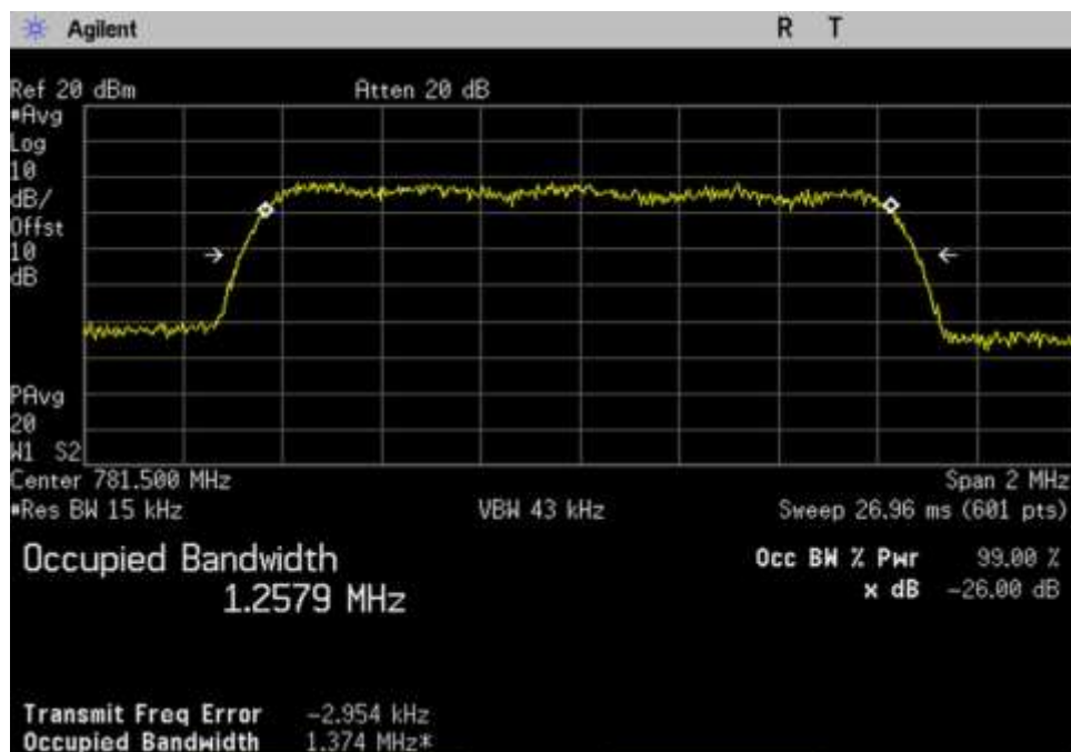
7.10 OBW-Out_UL_776-787_CDMA_781.5MHz
