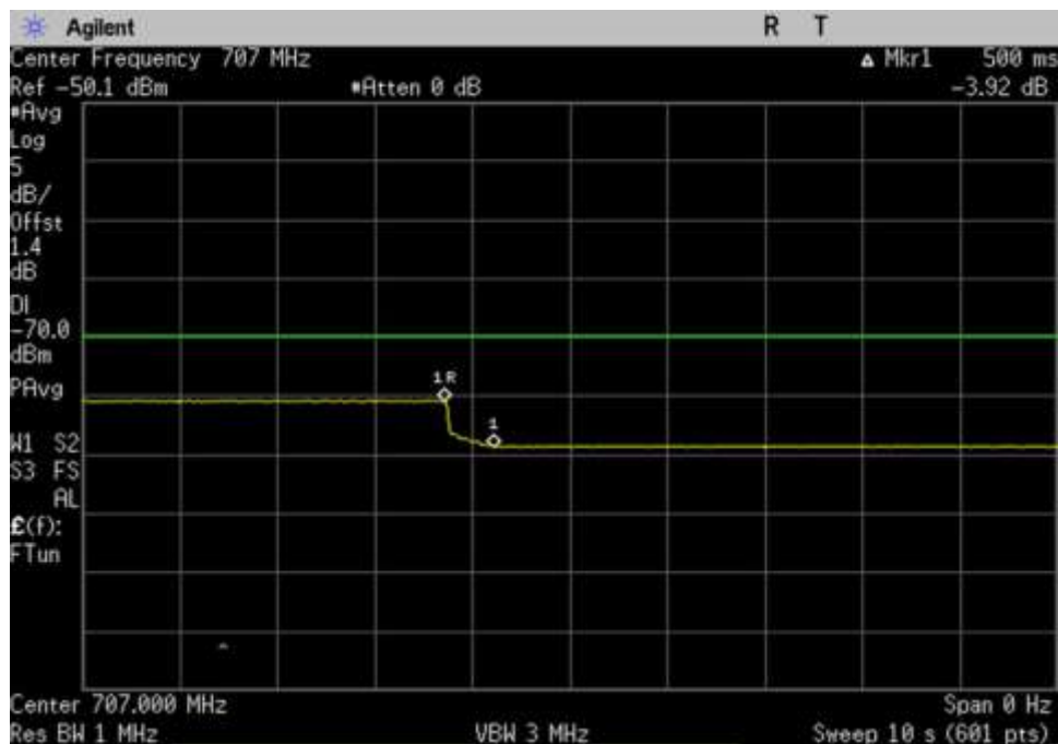
7.7 Noise_UL_698-716_707MHz_Timing
