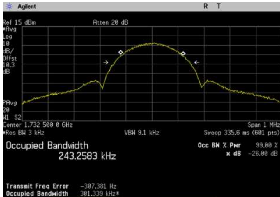
7.10 OBW-Out_UL_1710-1755_EDGE_ 1732.5MHz
