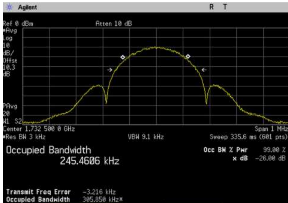
7.10 OBW-In_UL_1710-1755_EDGE_1732.5MHz
