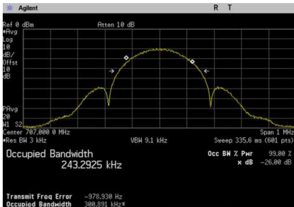
7.10 OBW-In_UL_698-716_EDGE_ 707MHz
