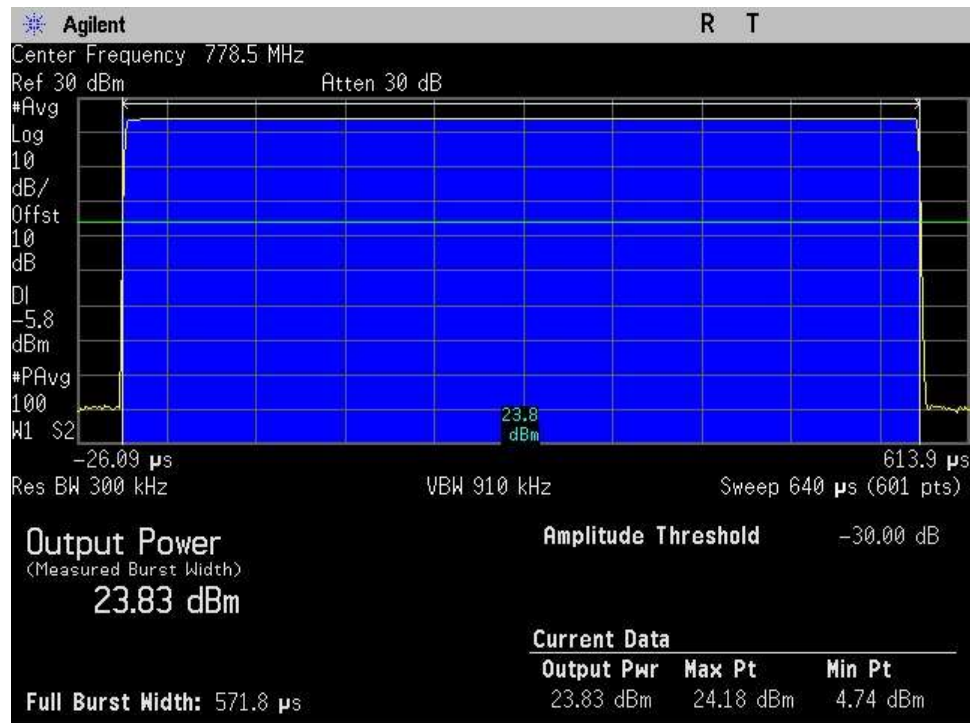
7.2-7.3 Power Gain_UL_776-787_GSM_ 778.5MHz
