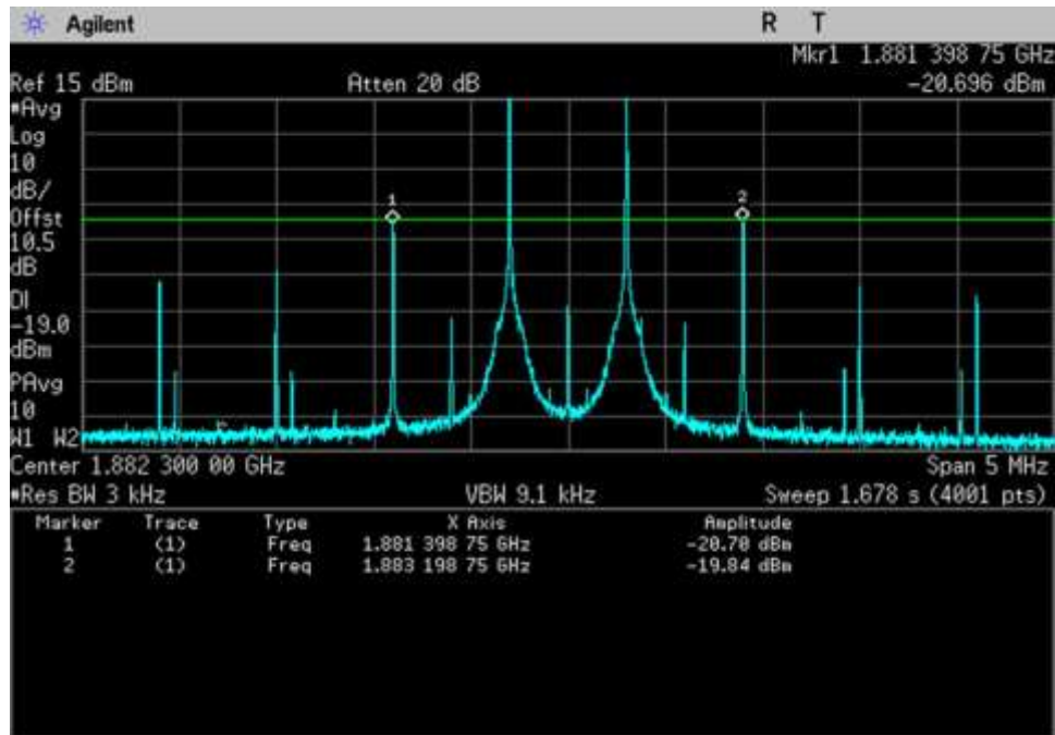
7.4 Intermod_UL_1850-1915_1882.3MHz
