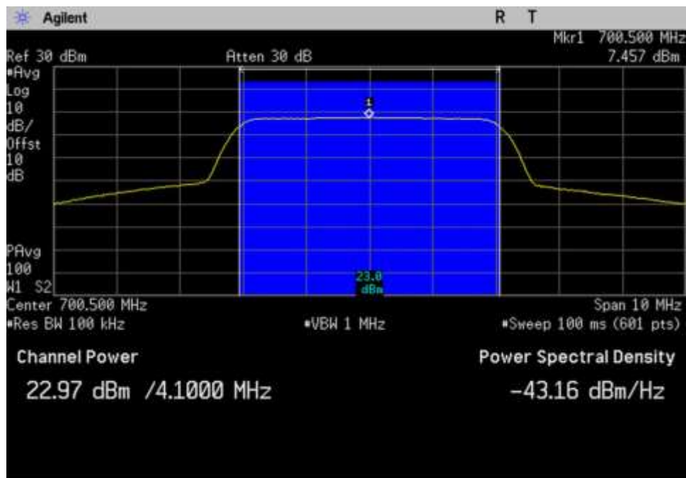
7.2-7.3 Power Gain_UL_698-716_AWGN_Max_ 700.5MHz
