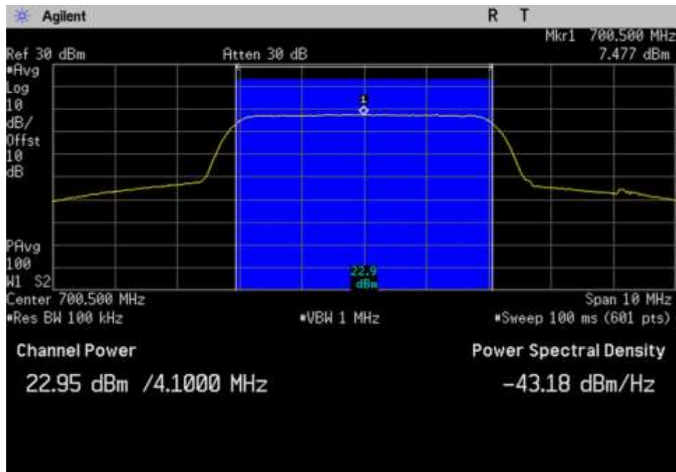
7.2-7.3 Power Gain_UL_698-716_AWGN_ 700.5MHz
