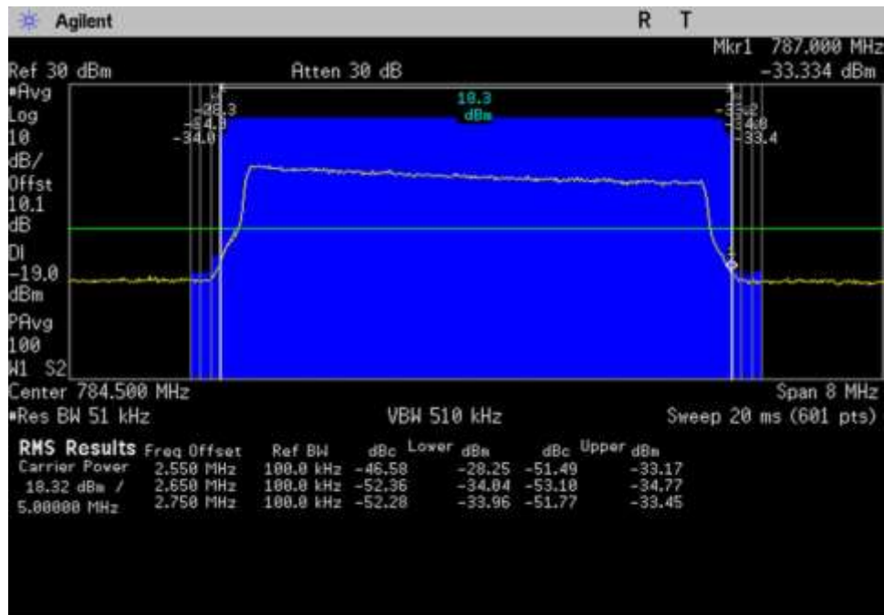
7.5 OBE_UL_776-787_LTE_780.5- 788.5MHz
