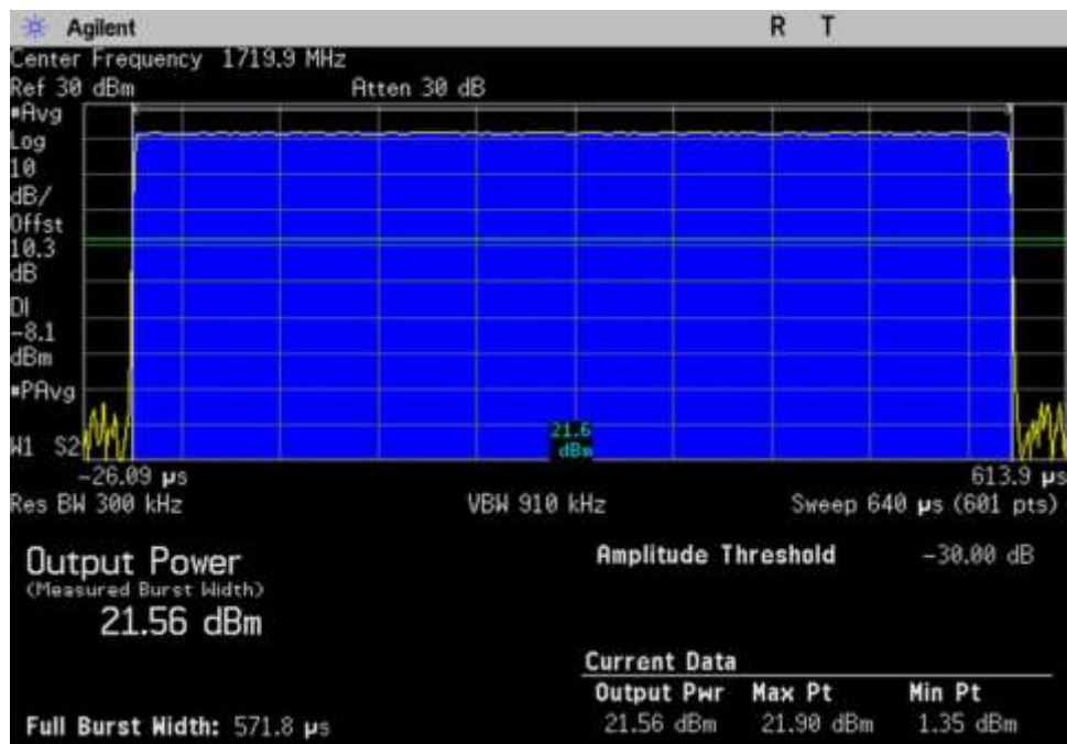
7.2-7.3 Power Gain_UL_1710-1755_GSM_Max_ 1719.9MHz
