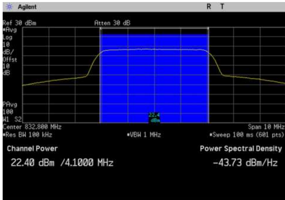
7.2-7.3 Power Gain_UL_824-849_AWGN_ 832.8MHz
