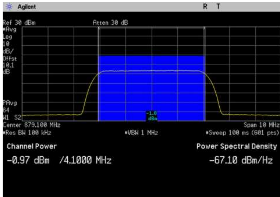
7.2-7.3 Power Gain_DL_869-894_AWGN_ 879.1MHz
