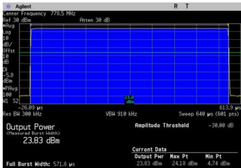
7.2-7.3 Power Gain_UL_776-787_GSM_Max_ 778.5MHz
