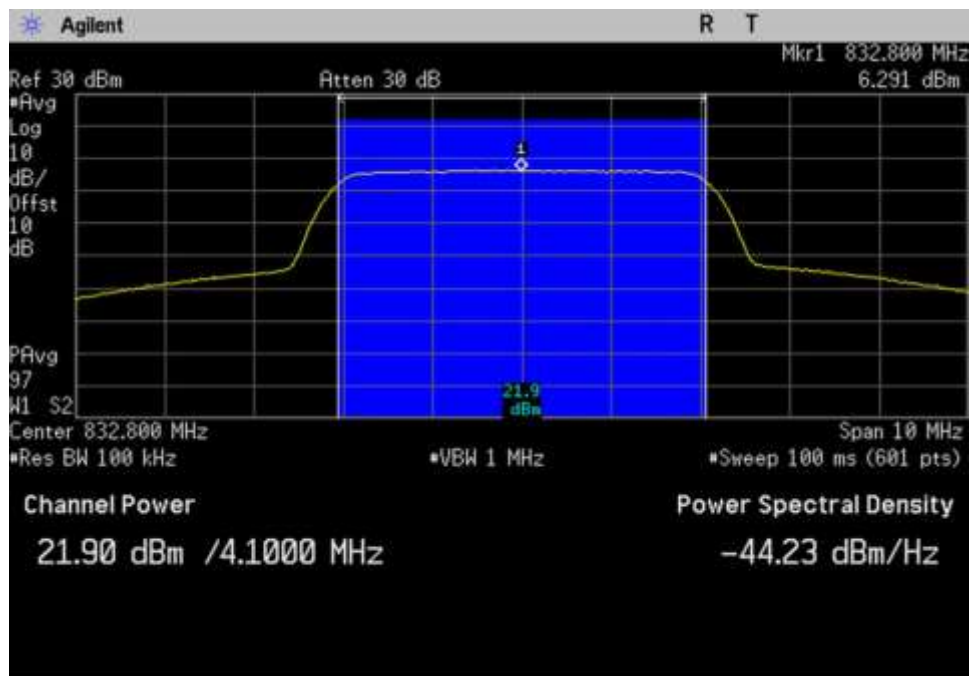
7.2-7.3 Power Gain_UL_824-849_AWGN_Max_ 832.8MHz
