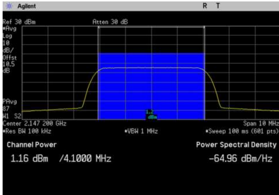
7.2-7.3 Power Gain_DL_2110-2155_AWGN_ 2147.2MHz
