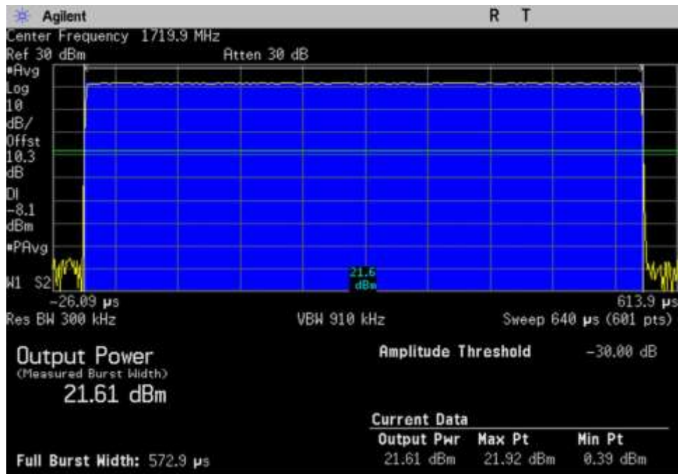
7.2-7.3 Power Gain_UL_1710-1755_GSM_ 1719.9MHz
