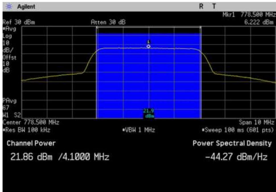
7.2-7.3 Power Gain_UL_776-787_AWGN_Max_778.5MHz
