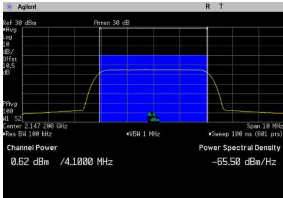
7.2-7.3 Power Gain_DL_2110-2155_AWGN_Max_ 2147.2MHz
