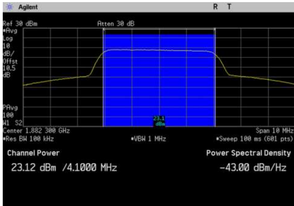
7.2-7.3 Power Gain_UL_1850-1915_AWGN_1882.3MHz
