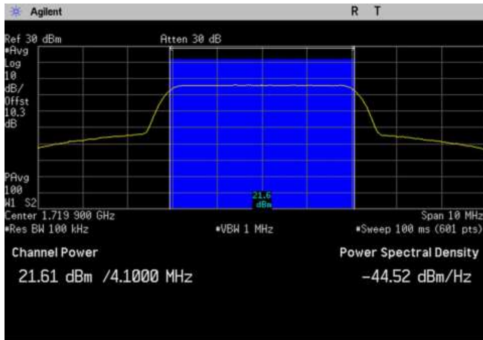
7.2-7.3 Power Gain_UL_1710-1755_AWGN_1719.9MHz
