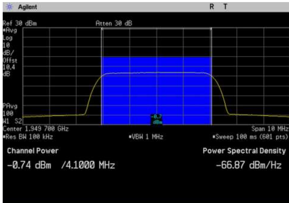
7.2-7.3 Power Gain_DL_1930-1995_AWGN_ 1949.7MHz
