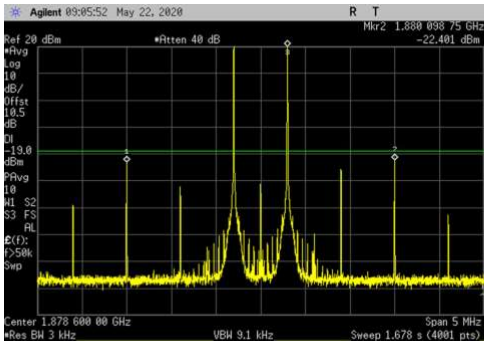
UL_1850-1915_1878.6MHz
