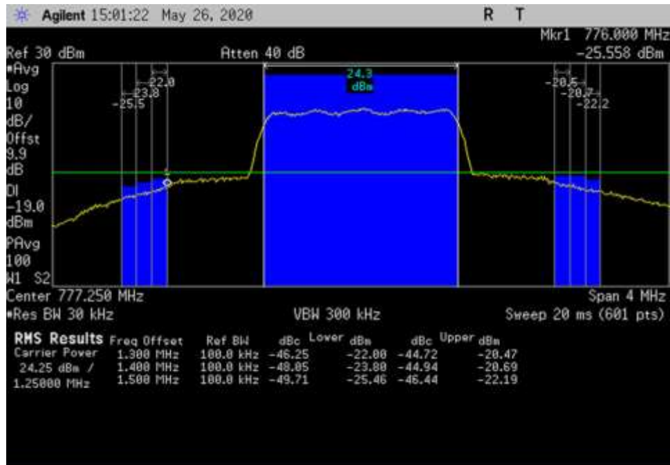
UL_776-787_CDMA_775.25- 779.25MHz
