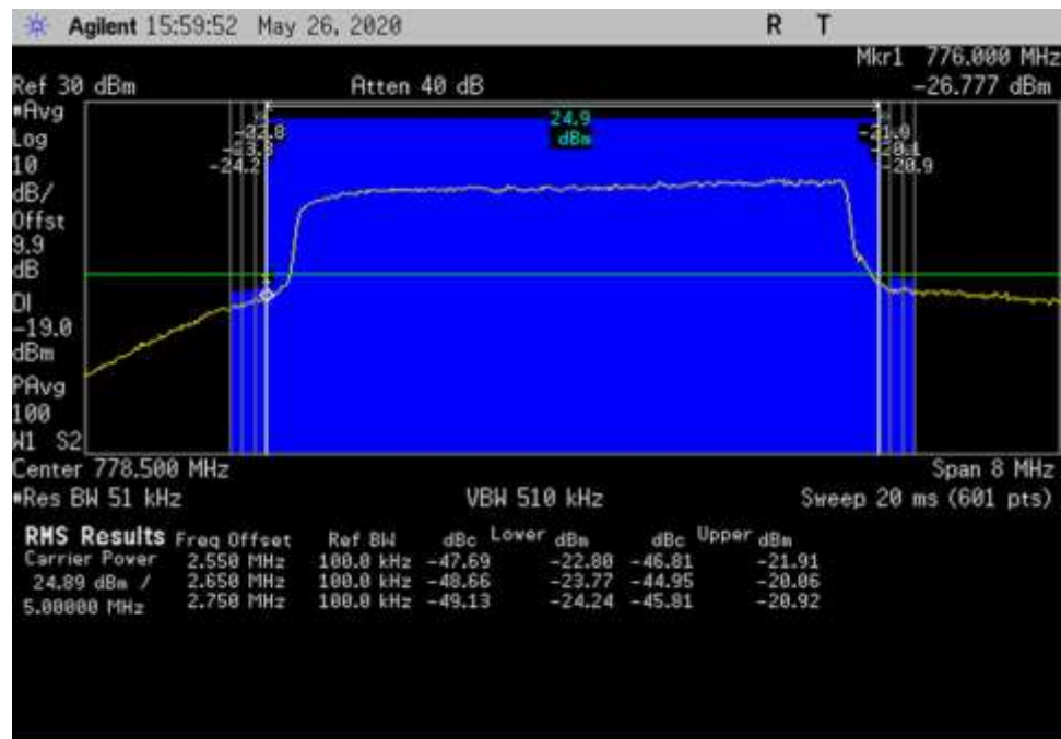
UL_776-787_LTE_774.5- 782.5MHz
