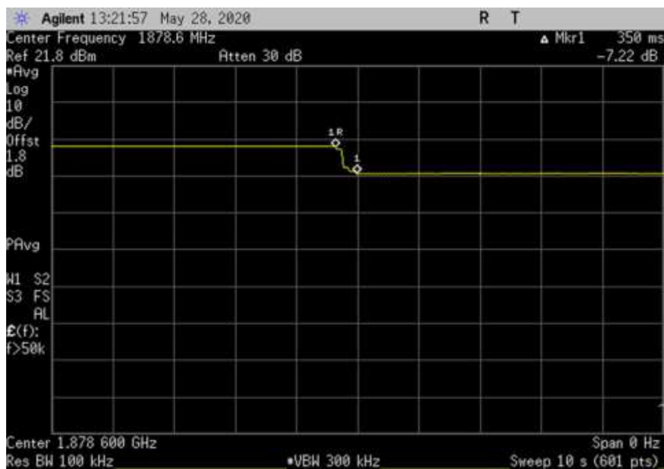
UL_1850-1915_ 1878.6MHz_Timing
