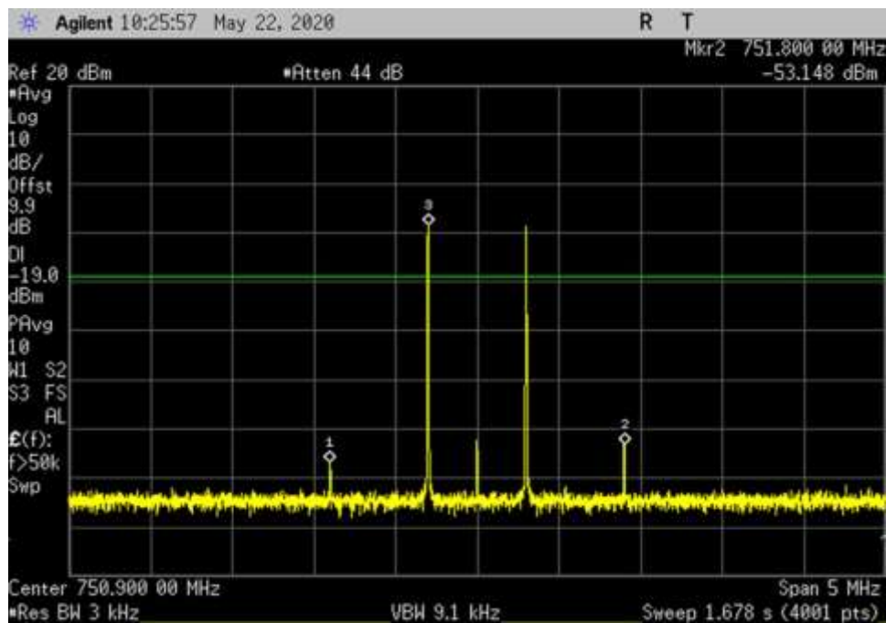
DL_746-757_ 750.9MHz
